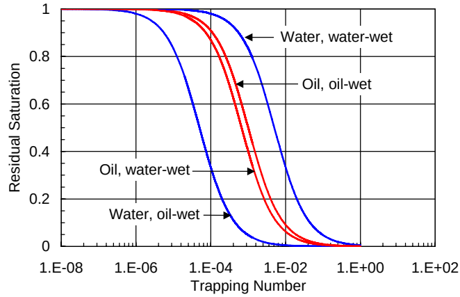
Fig. 1—Capillary desaturation curves used in simulations.
