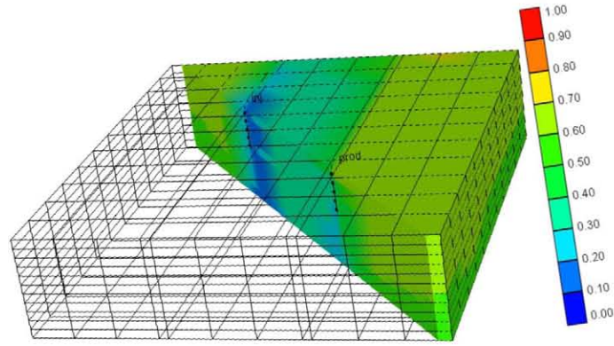
Fig. 7—Oil saturation at 1200 days of surfactant injection (wettability alteration case with \omega = 0.5 ).
