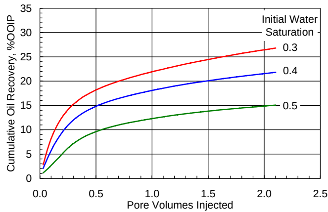
Fig. 11—Effect of initial water saturation in matrix during surfactant flood with wettability alteration.
