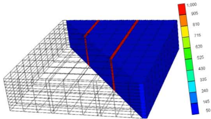
Fig. 5—Schematic of grid and permeability (md) for 3-D simulations.
