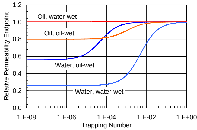
Fig. 2—Endpoint relative permeability.
