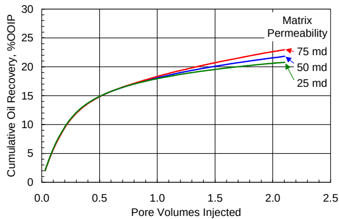
Fig. 12—Effect of matrix permeability during surfactant flood with wettability alteration.
