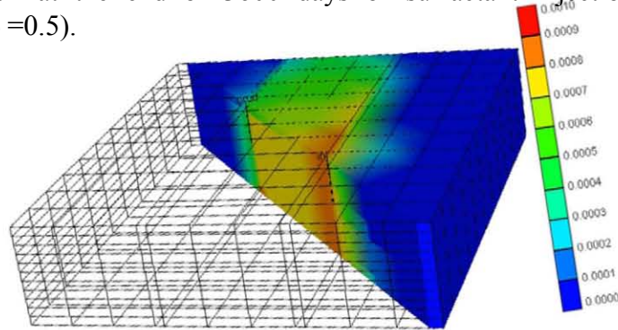
Fig. 9—Surfactant concentration in volume fraction at the end of 3600 days of surfactant injection (wettability alteration case with \omega = 0.5 ).
