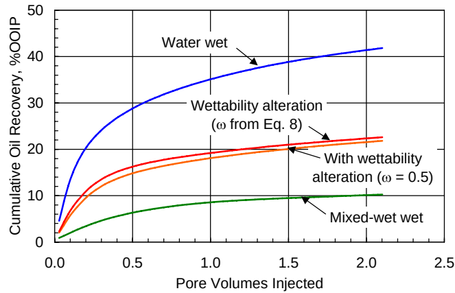
Fig. 10—Surfactant flood oil recovery in fractured reservoir at different wettability conditions.
