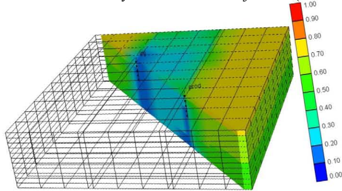
Fig. 8—Oil saturation at the end of 3600 days of surfactant injection (wettability alteration case with \omega = 0.5 ).
