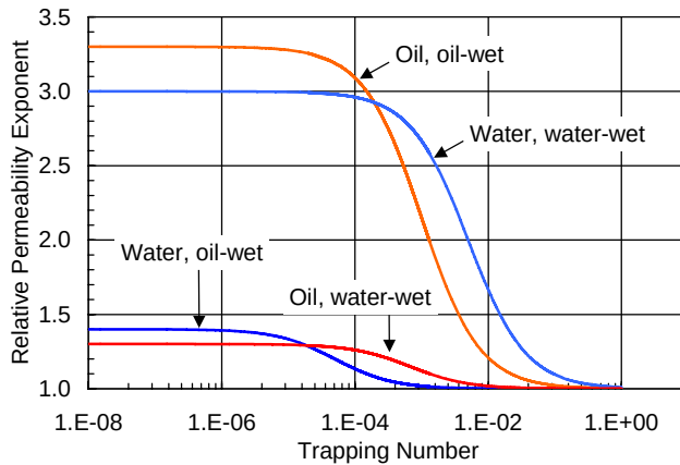
Fig. 3—Relative permeability exponent.
