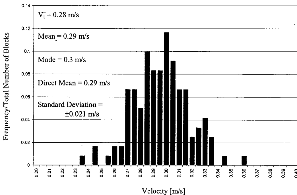
Figure 5. Local Velocity Distribution (65,536 Block Size)
