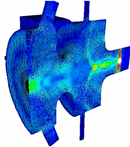
Figure 14. Beam transit in LCLS rf gun using Pic3P
