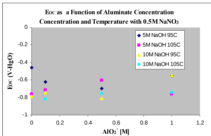
Figure 21: E_{OC} as a function of Aluminate in 0.5M \text{NaNO}_3/\text{NaOH} Solutions.
