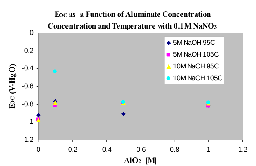
Figure 20: E_{OC} as a Function of Aluminate in 0.1M \text{NaNO}_3/\text{NaOH} Solutions
