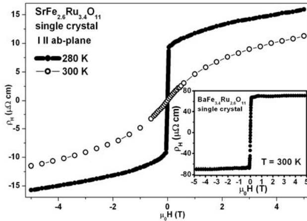
Fig. 6. Magnetic field dependence of the Hall resistivity \rho_H(H) of single-crystal \text{SrFe}_{2.6}\text{Ru}_{3.4}\text{O}_{11} at 280 and 300 K. The sharp change in slope at 0.1 T (anomalous Hall effect) is proof of spontaneous electron spin-polarization. Inset shows \rho_H(H) for single-crystal \text{BaFe}_{3.4}\text{Ru}_{2.6}\text{O}_{11} at T = 300 K. After [15,16].
