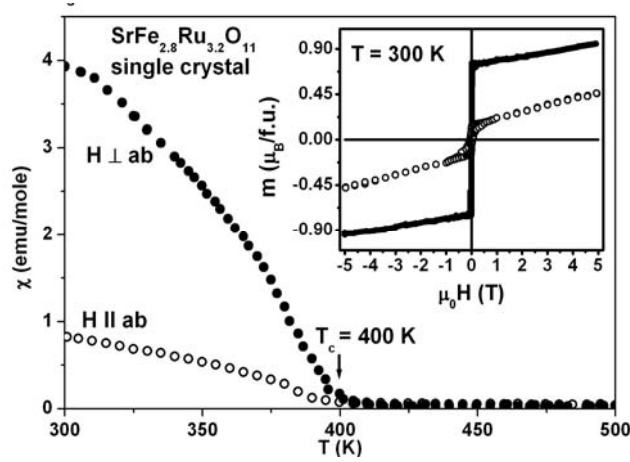
Fig. 2. Temperature dependence of the FC DC magnetic susceptibility \chi(T) of single-crystal \text{SrFe}_{2.8}\text{Ru}_{3.2}\text{O}_{11} for \mathbf{H} \parallel \mathbf{ab} and \mathbf{H} \perp \mathbf{ab} plane (easy direction) at applied magnetic field \mu_0 H = 0.1 T. Inset shows the magnetic moment m vs. H at 300 K for the two field orientations. Arrow designates the FM ordering temperature T_c . After [15,16].
