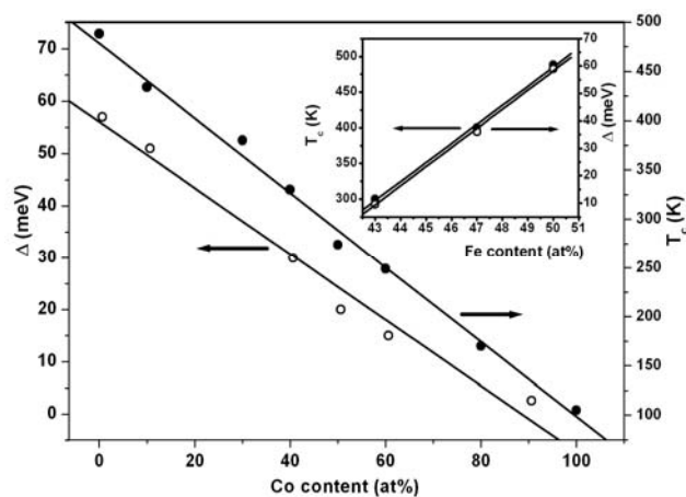
Fig. 9. Co concentration dependence of the Curie temperature T_C and semiconducting gap \Delta for polycrystalline Sr(Fe 1-y Co y ) 2±x Ru 4±x O 11 solid solutions having nominal compositions 0 \leq y \leq 1 , x = 0 . Inset: Fe concentration dependence of T_C and \Delta for SrFe 2+x Ru 4-x O 11 ( x = 0.6, 0.8 single crystals, x = 1 polycrystal). Solid lines are linear fits to the data. After [15].
