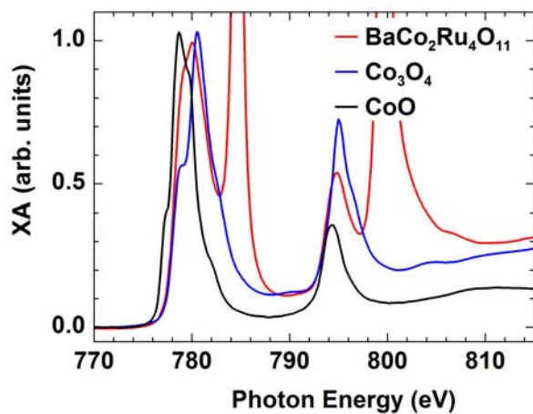
Fig. 8. Co XA spectra of Co +2 (Co +3 ) 2 O 4 , Co +2 O and BaCo 2 Ru 4 O 11 showing the Co oxidation state in the latter material is mixed (+2/+3). The pronounced spectral features near 785 eV and 800 eV in BaCo 2 Ru 4 O 11 are due to the Ba M 4,5 absorption edges.
