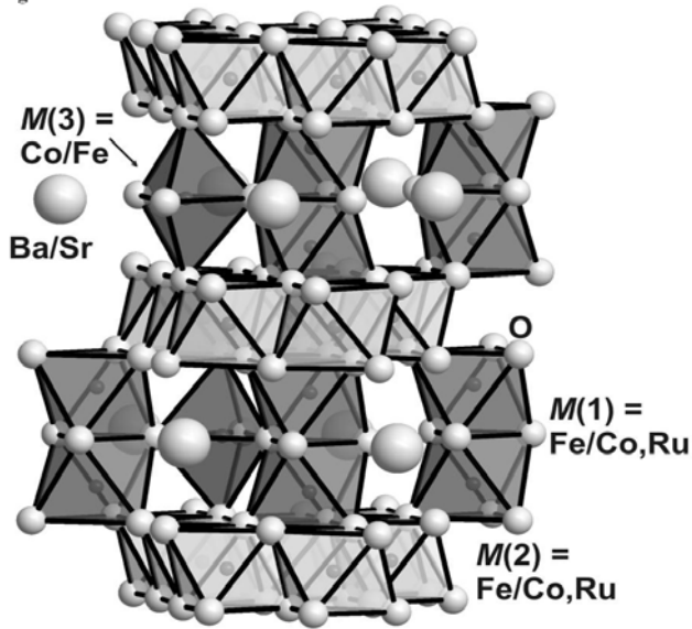
Fig. 1. (\text{Ba,Sr})\text{M}_{2\pm x}\text{Ru}_{4\pm x}\text{O}_{11} ( \text{M} = \text{Fe, Co} ) crystal structure: Layers of \text{M}(2)\text{O}_6 (octahedra) are connected in the [001] direction via \text{M}(1)_2\text{O}_9 double-octahedra and \text{FeO}_5 or \text{CoO}_5 trigonal prisms. Ba (Sr) (large spheres) is located within the layers of double-octahedra and trigonal prisms. After [14].
