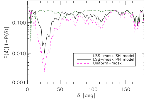
Figure 3: Chance probability of auto correlation taking as reference model an uniform distribution, the linear correlation model of [6] (LSS-PH model) and the presently considered model with a smaller horizon (LSS-SH model). See text for details.
