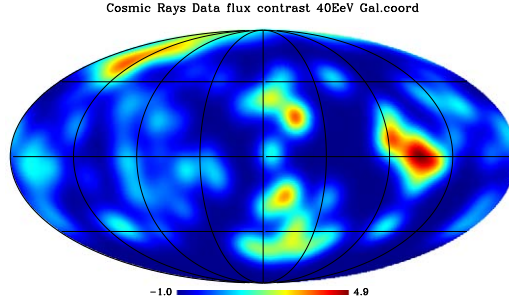
Figure 1: The UHECR flux contrast map (or excess map) properly smoothed with a Gaussian filter of 10^\circ width in galactic coordinates.
