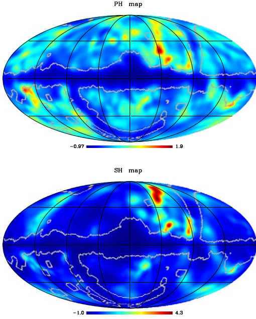
Figure 2: Excess maps of the LSS-PH (top panel) and LSS-SH models (bottom panel). The grey contour bounds the blind region of PSCz catalogue.
