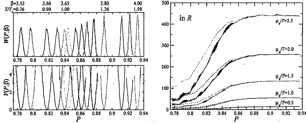
Figure 2: (left) The plaquette histogram and the effective potential at \mu_q = 0 . (right) The reweighting factor \ln R(P, \mu_q) for \mu_q/T = 0.5 - 2.5 .
