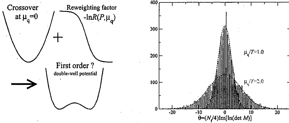
Figure 1: (left) Schematic figures of the effective potential and the reweighting factor. (right) The histogram of the complex phase for \mu_q/T = 1.0 and 2.0 at \beta = 3.65 .
