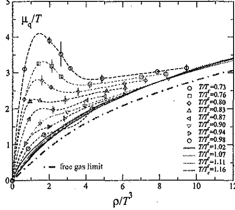
Figure 4: The chemical potential as a function of the quark number density.
