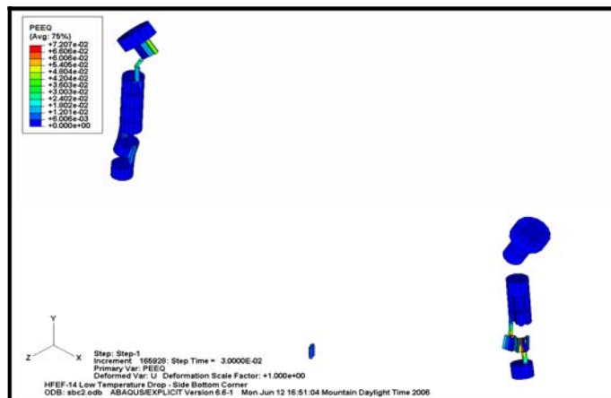
Figure 6. Plastic strain in the door bolts at the end of the analysis of the bottom corner drop. Note the elements removed after failure.
