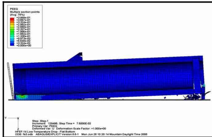
Figure 8. Flat side drop showing the lid separated from the cask and the shattered door structure elements.
