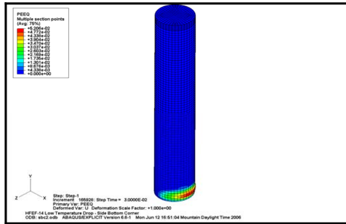
Figure 7. Plastic strain in the outer can from the bottom corner drop.
