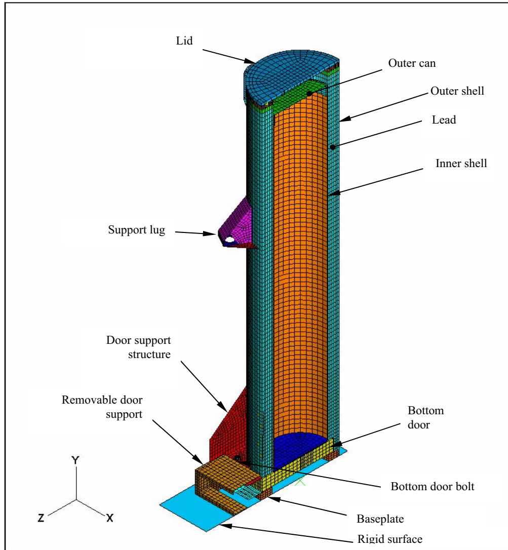
Figure 1. Cutaway view of the HFEF-14 cask showing various features.
