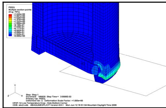
Figure 5. Cut away view of the plastic strain in the elements at the end of the bottom corner drop.
