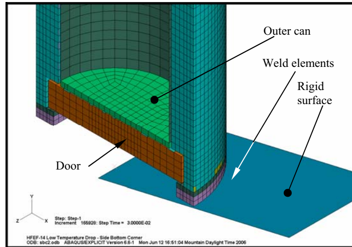
Figure 2. Cutaway view of the drop configuration for the side bottom corner drop.
