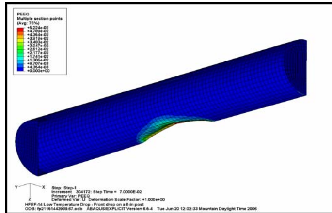
Figure 10. Indentation of the inner can from the side impact on a rigid post.
