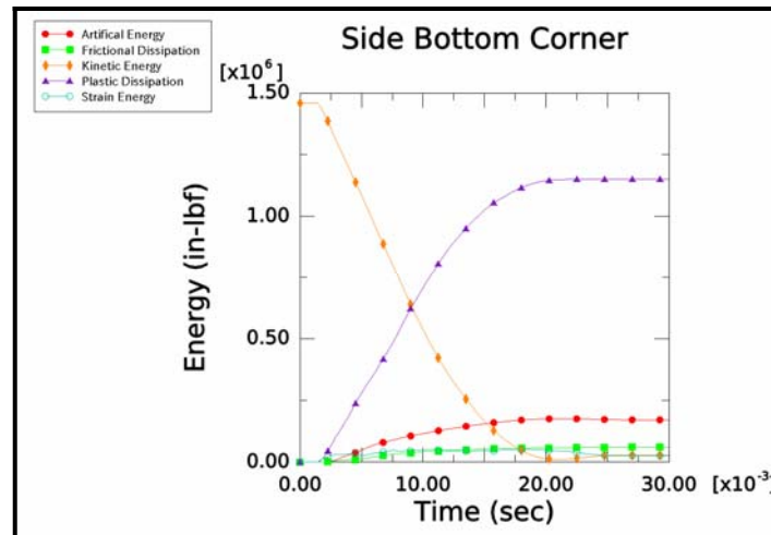
Figure 3. Energy expended during the bottom corner drop drop.
