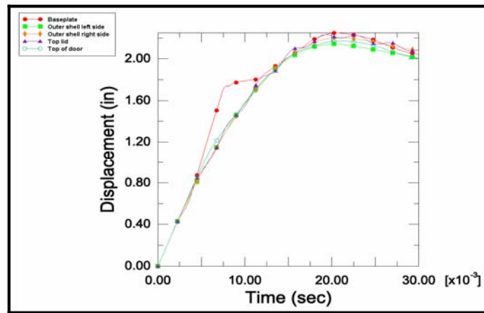
Figure 4. Displacement of various nodes during the bottom corner drop.
