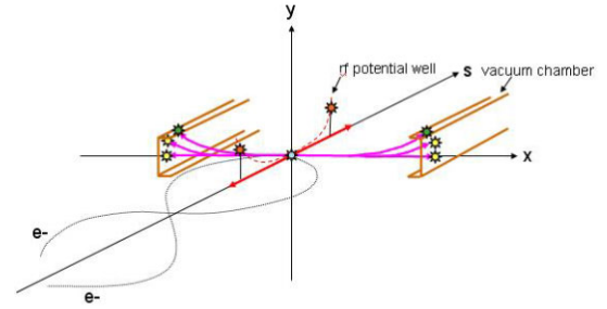
Figure 1: Touschek scattering loss mechanisms.
