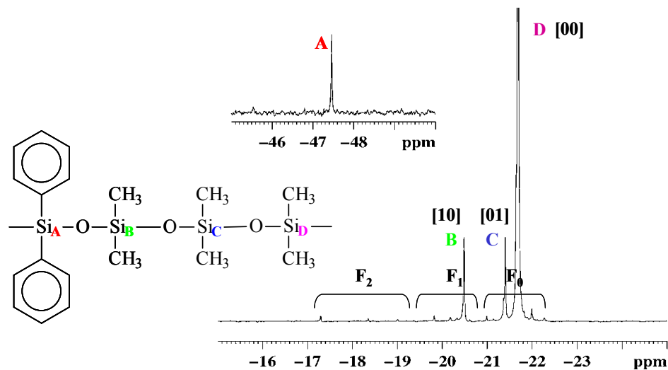
Figure 1: High-resolution ^{29}\text{Si} of HVM97 in \text{CDCl}_3 at 60 °C
