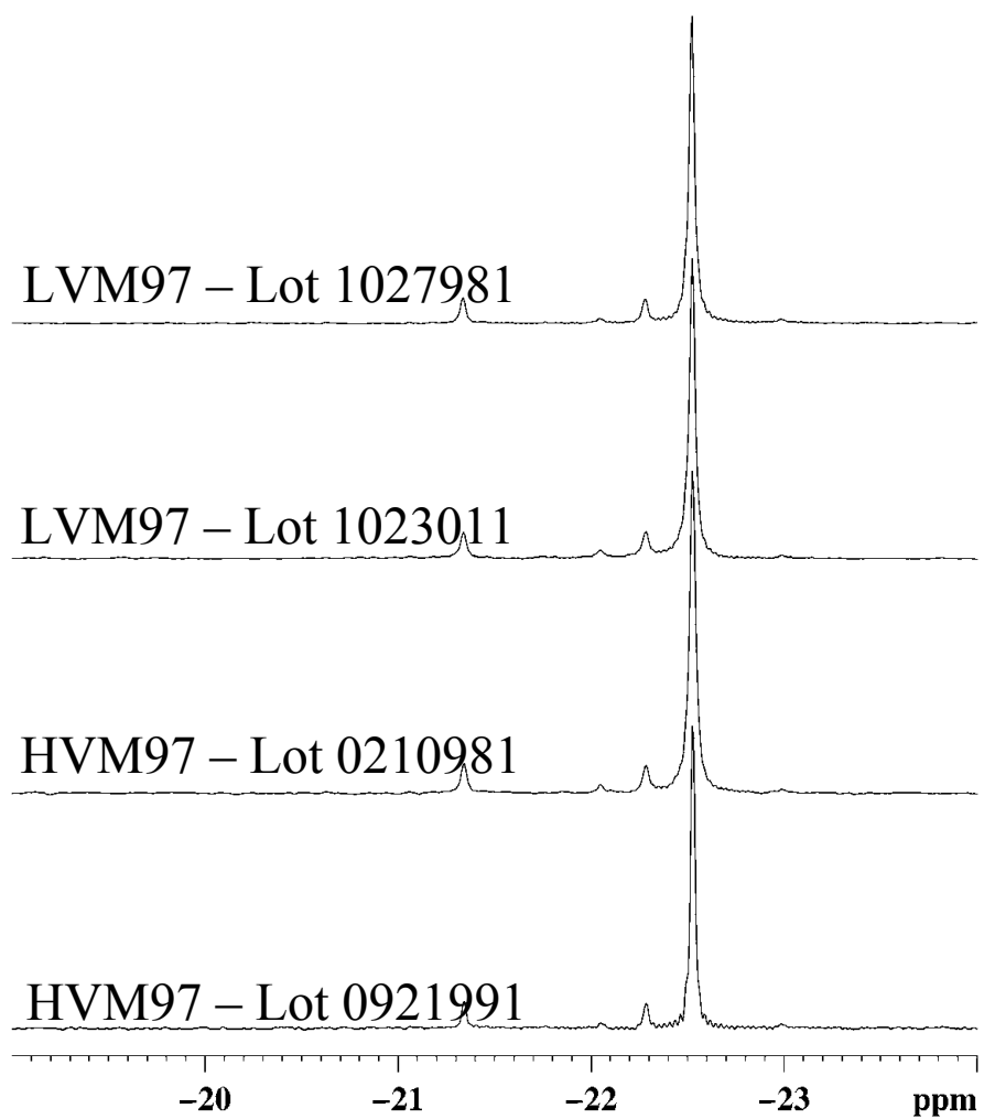
Figure 2: High-resolution ^{29}\text{Si} NMR for different production lots of LVM97 and HVM97.
