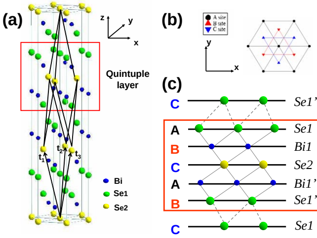
FIG. 1: Crystal Structure (a) Crystal structure of Bi_2Se_3 with three primitive lattice vectors denoted as \vec{t}_{1,2,3} . A quintuple layer with Se1 - Bi1 - Se2 - Bi1' - Se1' is indicated by the red box. (b) Top view along the z direction. Triangle lattice in one quintuple layer has three different positions, denoted as A, B and C. (c) Side view of the quintuple layer structure. Along z direction, the stacking order of Se and Bi atomic layers is the sequence \dots - C(Se1') - A(Se1) - B(Bi1) - C(Se2) - A(Bi1') - B(Se1') - C(Se1) - \dots . Se1 ( Bi1 ) layer can be related to Se1' ( Bi1' ) layer by an inversion operation of which Se2 atoms play the role of inversion center.
