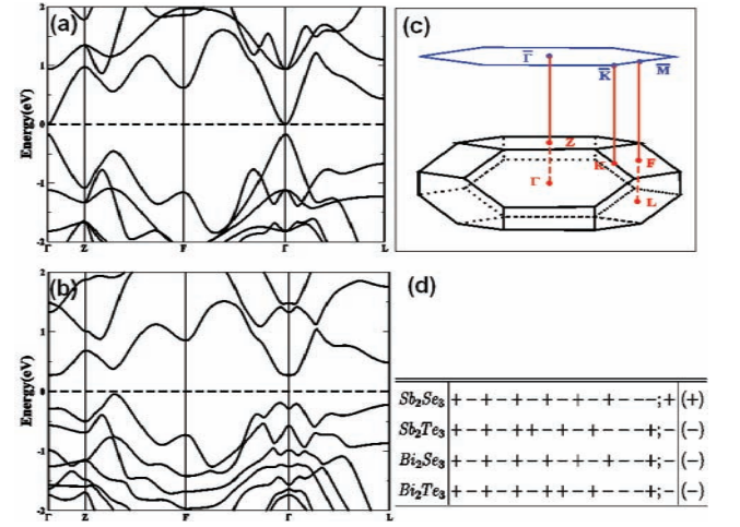
FIG. 2: band structure, Brillouin zone and parity eigenvalues. Band structure for Bi_2Se_3 without spin-orbit coupling(SOC) (a) and with SOC (b). The dashed line indicates Fermi level. (c) BZ for Bi_2Se_3 with space group R\bar{3}m . The four inequivalent time-reversal invariant points are \Gamma(0,0,0) , L(\pi,0,0) , F(\pi,\pi,0) and Z(\pi,\pi,\pi) . The blue hexagon shows the 2D BZ of projected (1,1,1) surface, in which the high-symmetry k points \bar{\Gamma} , \bar{K} and \bar{M} are labeled. (d) The parity of the band at \Gamma point for the four materials Sb_2Te_3 , Sb_2Se_3 , Bi_2Se_3 and Bi_2Te_3 . Here we show the parities of fourteen occupied bands, including five s bands and nine p bands, and the lowest unoccupied band. The product of the parities for the fourteen occupied bands is given in the bracket on the right of each row.
