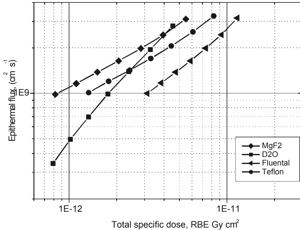
Fig. 1. The computed results obtained in investigations for readily available moderator materials: namely, heavy water, magnesium fluoride, polytetrafluoroethylene and Flualtal®.
