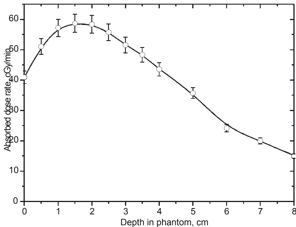
Fig. 4. Comparison of absorbed doses between calculation results (line) and experimental measurements (points) is shown.
