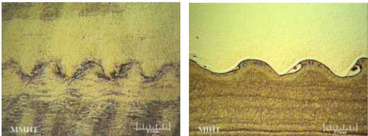
Figure 4. Optical micrographs of the interface of an explosion weld between (a) MA956 and MA956 plate and (b) MA956 and 601 plate.
