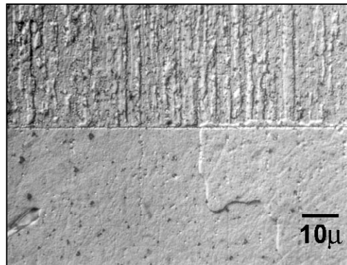
Figure 3. Joint produced using transient liquid phase bonding.
