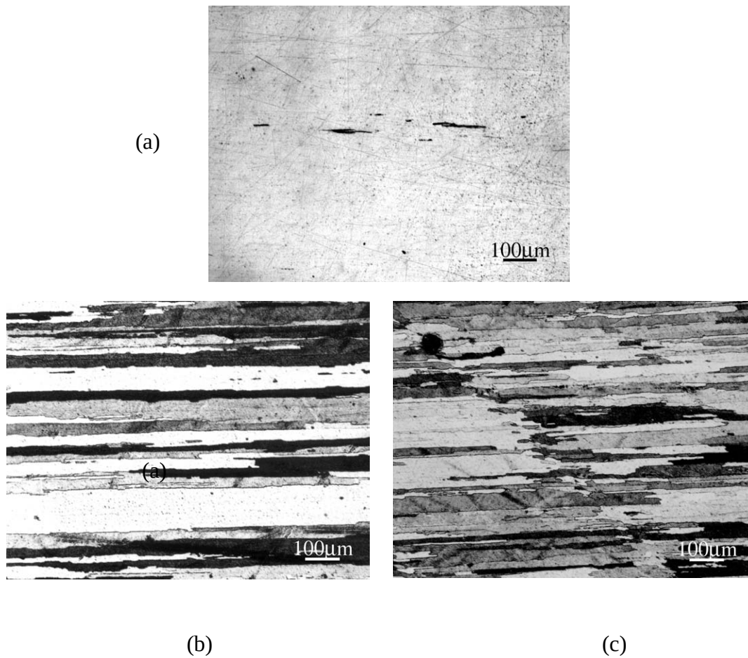
Figure 1. Variation in microstructure for MA956 rods extruded at 1000°C using a 20:1 extrusion ratio followed by (a) 0% CW, (b) 10% CW, and (c) 30% CW, and then annealed at 1300°C for 6 hours.
