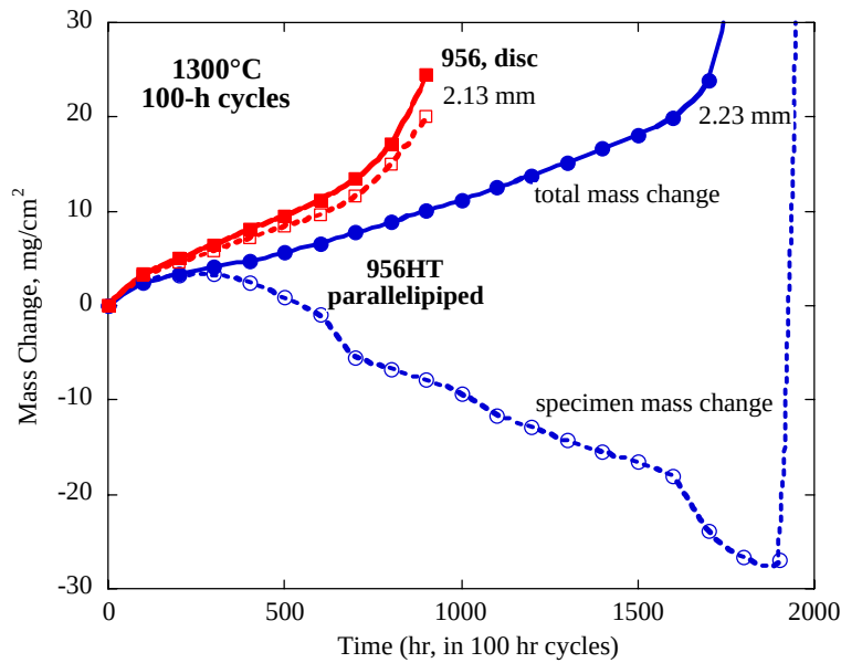
Figure 5. Plot of total mass change (solid line) and specimen mass change (dotted line) for the MA956 and MA956HT alloys oxidized in air at 1300°C.
