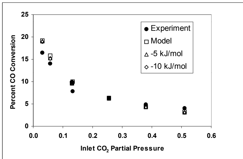
Figure 3. Effect of \text{CO}_3^* bond strength upon WGS inhibition by \text{CO}_2 .
