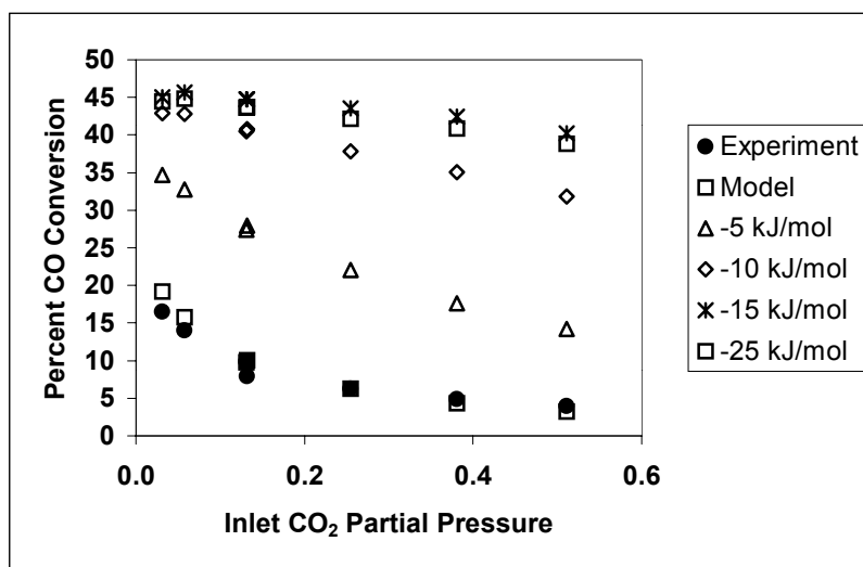
Figure 4. Effect of \text{O}^* bond strength upon WGS inhibition by \text{CO}_2 .
