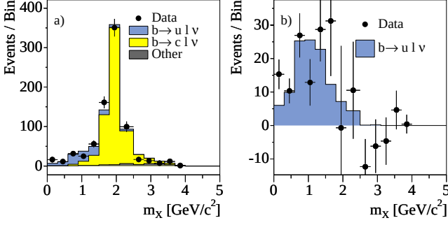
FIG. 1: The m_X distribution for \bar{B} \rightarrow X \ell \bar{\nu} candidates: a) data (points) and fit components after the minimum- \chi^2 fit, and b) data and signal MC after subtraction of the \bar{B} \rightarrow X_c \ell \bar{\nu} and other backgrounds. The upper edge of the eighth bin is chosen to be at m_X = 2.5 \text{ GeV}/c^2 . This fit result, with \chi^2 = 10.2 for 11 degrees of freedom, is used to extract the number of signal events below 2.5 \text{ GeV}/c^2 .
