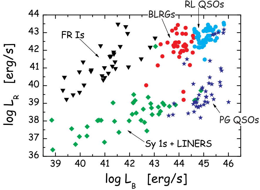
Figure 1. L_R vs. L_B for the analyzed sample.
