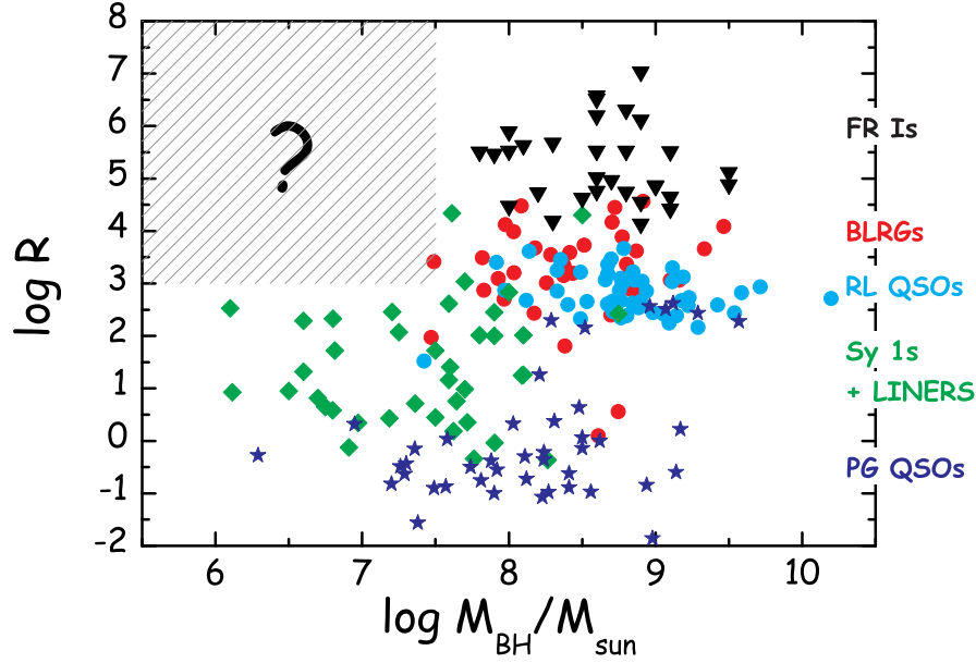
Figure 4. \mathcal{R} vs. \mathcal{M}_{\text{BH}} for the analyzed sample.
