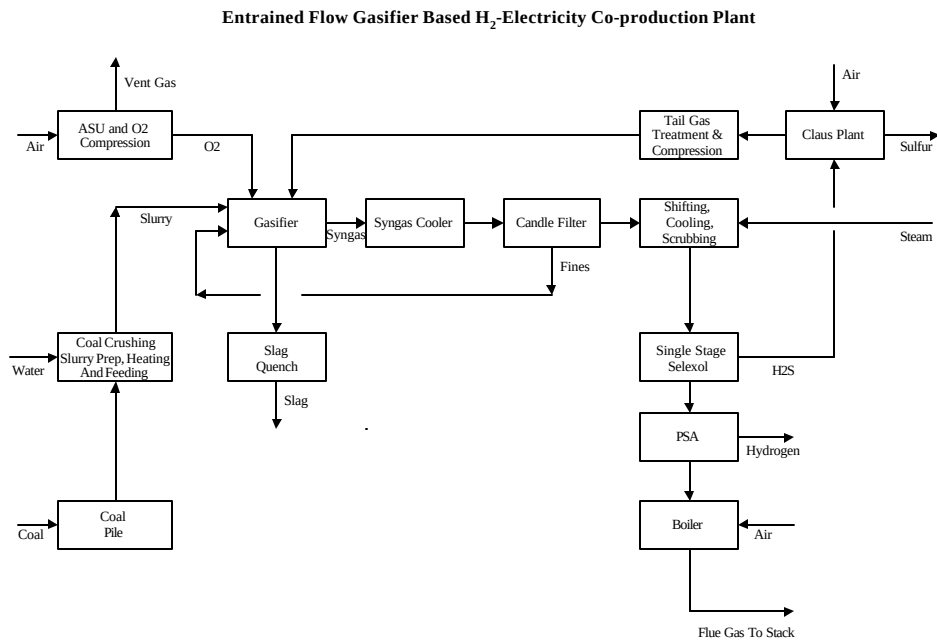
Figure 3 Entrained Flow Co-production Plant Block Diagram (Single Gasification Train)
