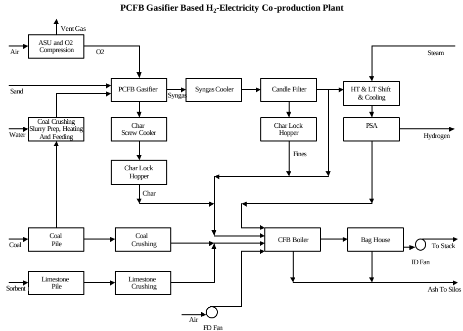
Figure 4 PGM Co-production Plant Block Diagram
