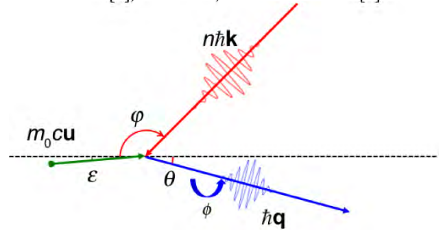
Figure 1: Interaction geometry.
