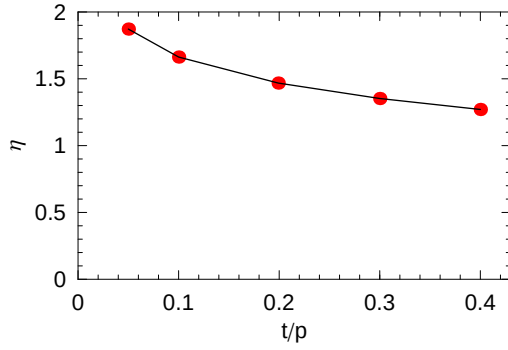
Figure 4: For the vacuum chamber with rounded fin tips: the enhancement factor \eta as function of t/p (the plotting symbols).
