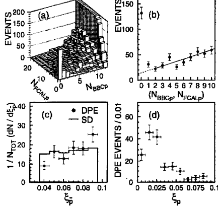
Fig. 1. (a) BBC hit multiplicity versus forward calorimeter tower multiplicity on the p side, (b) multiplicity distribution along the diagonal bins in (a), (c) \xi_{\bar{p}} measured by RPS for the DPE (points) and SD (histogram) events, (d) \xi_p of the DPE events.
