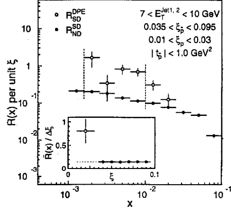
Fig. 2. Ratios of DPE to SD (SD to ND) dijet event rates per unit \xi_p ( \xi_{\bar{p}} ), shown as open (filled) circles, as a function of x_p ( x_{\bar{p}} ). The insert shows the weighted average of ratios within the vertical dashed lines per unit \xi versus \xi .
