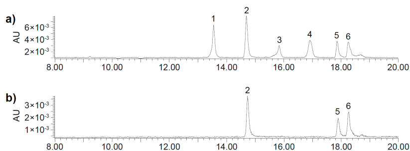
Figure 3. Exemplary UHPLC-DAD chromatograms of TBA isomers (450 nm) in (a) a model system containing \alpha -alanine and CQA at pH 9 and in (b) a model solution containing \alpha -alanine and PPO at pH 7.
