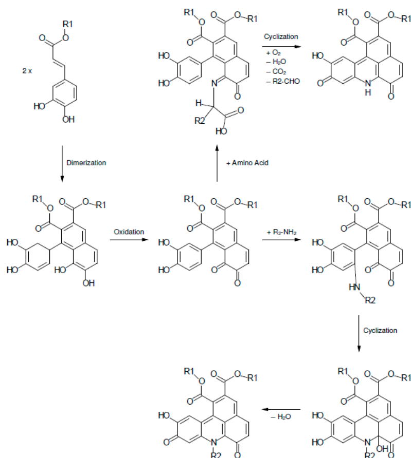
Figure 7. Proposed reaction mechanism between CQA and individual amino acids. If an \alpha - \text{NH}_2 group is involved, the resulting TBA core is free from any amino acid side chain. If TBA formation occurs at \beta - or \epsilon - \text{NH}_2 groups, corresponding amino acid side chains remain attached. \text{R}_1 = Quinic acid. \text{R}_2 = amino side chain.
