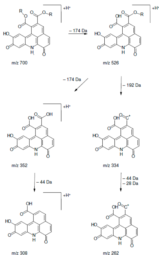
Figure 4. Postulated fragmentation pathway of a chlorogenic L-lysine adduct. R = Quinic acid Modified from [15].
