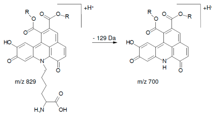
Figure 5. Postulated fragmentation of the chlorogenic L-lysine adduct with m/z 829 to the chlorogenic L-lysine adduct with m/z 700. R = Quinic acid. Modified from [15].
