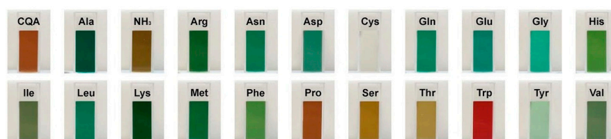
Figure 2. Color development in model systems containing CQA and individual amino acids at pH 9.
