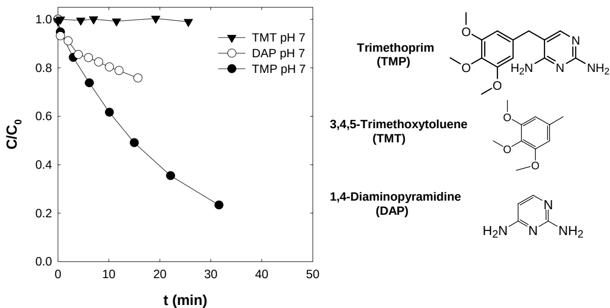
Figure 3.4. Mn(VII) oxidation of trimethoprim (TMP) in comparison to two analogues that represent sub-structural moieties within the TMP structure. Experimental conditions: C_0 = 10 \mu M, [Mn(VII)] _0 = 500 \mu M, 25 ^{\circ} C, pH 7, 25 mM phosphate buffer.
