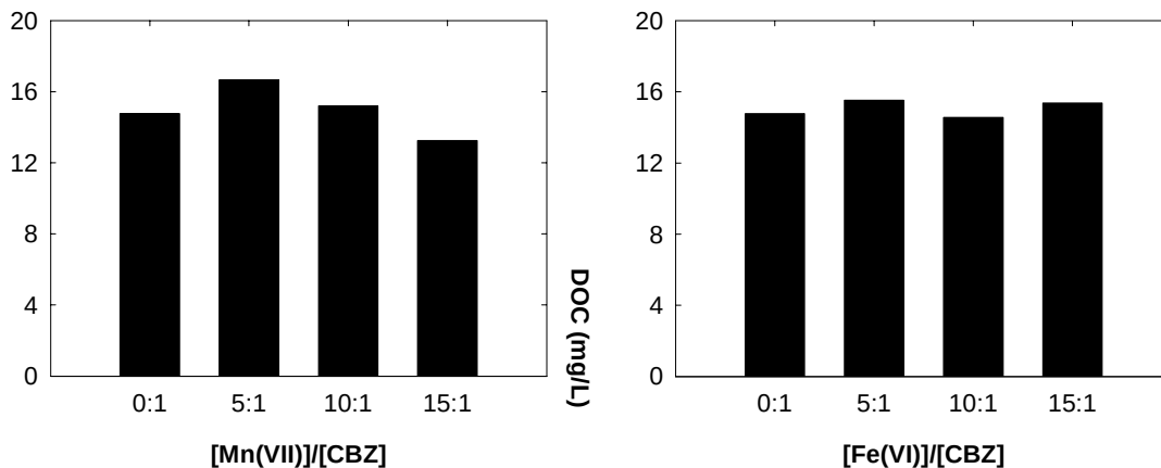
Figure 2.4. Dissolved organic carbon remaining in CBZ solutions following treatment with Mn(VII) and Fe(VI). Reaction condition: [CBZ] 0 = 80 \mu M, varying [Mn(VII)] and [Fe(VI)], pH 7.0 (25 mM phosphate buffer), 25 ^{\circ} C. Reactions were allowed to run for >10 h to reach completion before filtering (0.2 \mu m PTFE) and analyzing.
