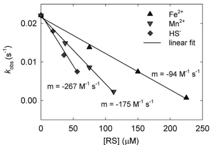
Figure 2.7. Effect of reduced species (RS) on the rate of CBZ oxidation by Mn(VII).
