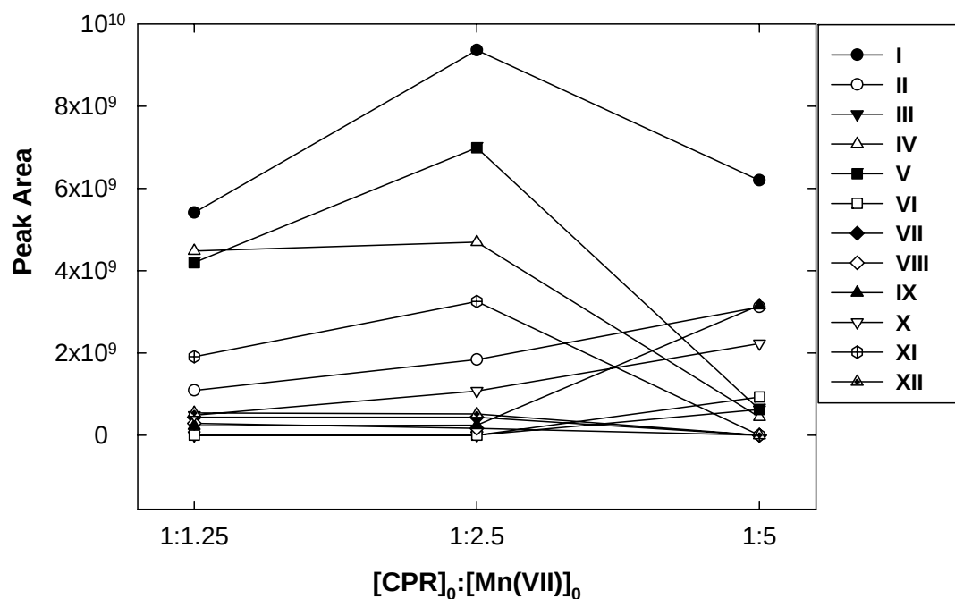
Figure 4.6. Integrated LC-MS peak areas of products from CPR reactions with Mn(VII): [\text{CPR}]_0 = 160 \mu\text{M} , pH 7 (25 mM ammonium acetate), 25 °C.
