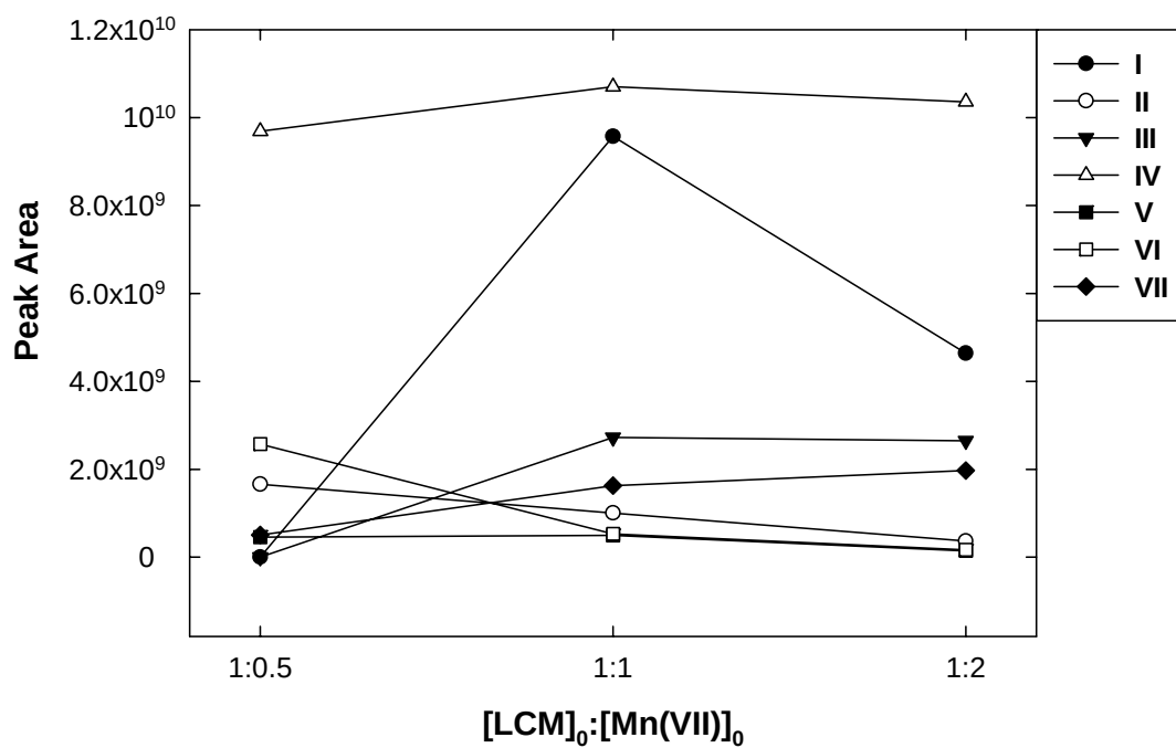
Figure 4.7. Integrated LC-MS peak areas of products from LCM reactions with Mn(VII): [\text{LCM}]_0 = 400 \mu\text{M} , pH 7 (25 mM ammonium acetate), 25 °C.
