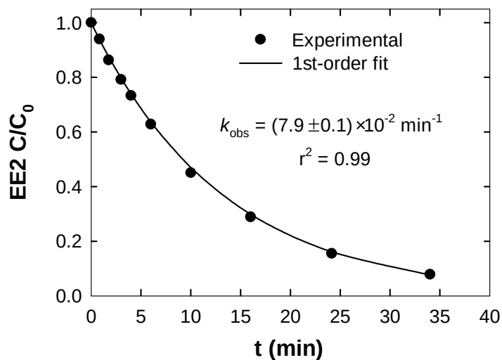
Figure 5.1. Representative batch reaction for oxidation of EE2 by excess concentrations of Mn(VII) and pseudo-first-order rate law model fit. Experimental conditions: [EE2]_0 = 1 \text{ } \mu\text{M} , [Mn(VII)]_0 = 10 \text{ } \mu\text{M} , 25 \text{ } ^\circ\text{C} , pH 7, 25 mM NaCl. Uncertainty represents 1 \sigma .
