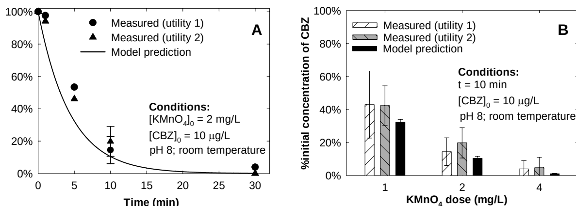
Figure 2.8. Comparison of kinetic model predictions and measured removal of CBZ during treatment of utility source waters with \text{KMnO}_4 : (A) Removal of CBZ as a function of time in source waters treated with 2 mg/L \text{KMnO}_4 ; (B) Removal of CBZ after 10 min in source waters dosed with different concentrations of \text{KMnO}_4 . CBZ concentrations reported relative to Mn(VII)-free control samples, where negligible CBZ degradation is observed. Uncertainties indicated by 1 SD provided when replicate samples measured.
