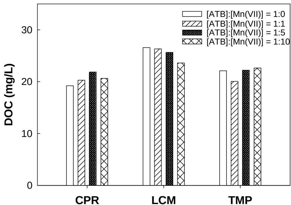
Figure 4.1. Measured dissolved organic carbon (DOC) concentration of the target antibiotics after treatment with different doses of Mn(VII). Reaction conditions: [ATB]_0 = 100 \mu\text{M} , varying [Mn(VII)] , 25 mM phosphate buffer, pH 7, room temperature.
