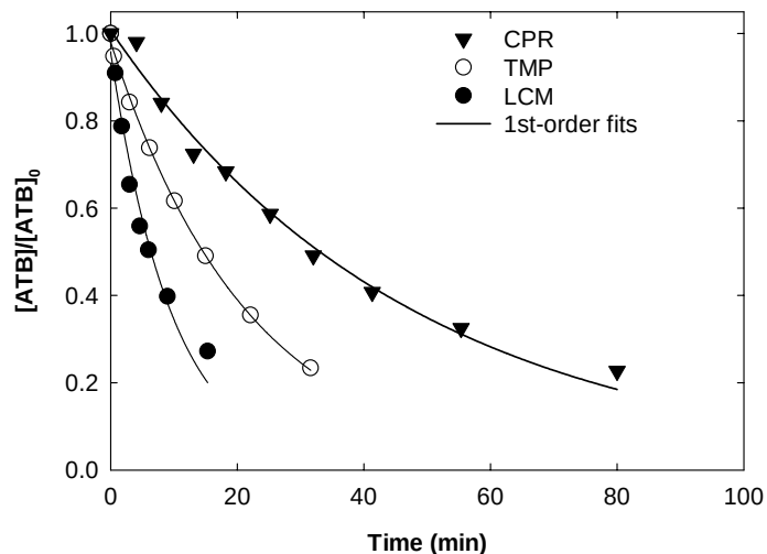
Figure 3.1. Oxidation of antibiotics by Mn(VII) during batch reactions and pseudo-first-order model fits. Experimental conditions: [\text{CPR}]_0 = 10 \mu\text{M} , [\text{LCM}]_0 = 20 \mu\text{M} , [\text{TMP}]_0 = 10 \mu\text{M} , [\text{Mn(VII)}]_0 = 500 \mu\text{M} , 25^\circ\text{C} , pH 7, 25 mM phosphate buffer.
