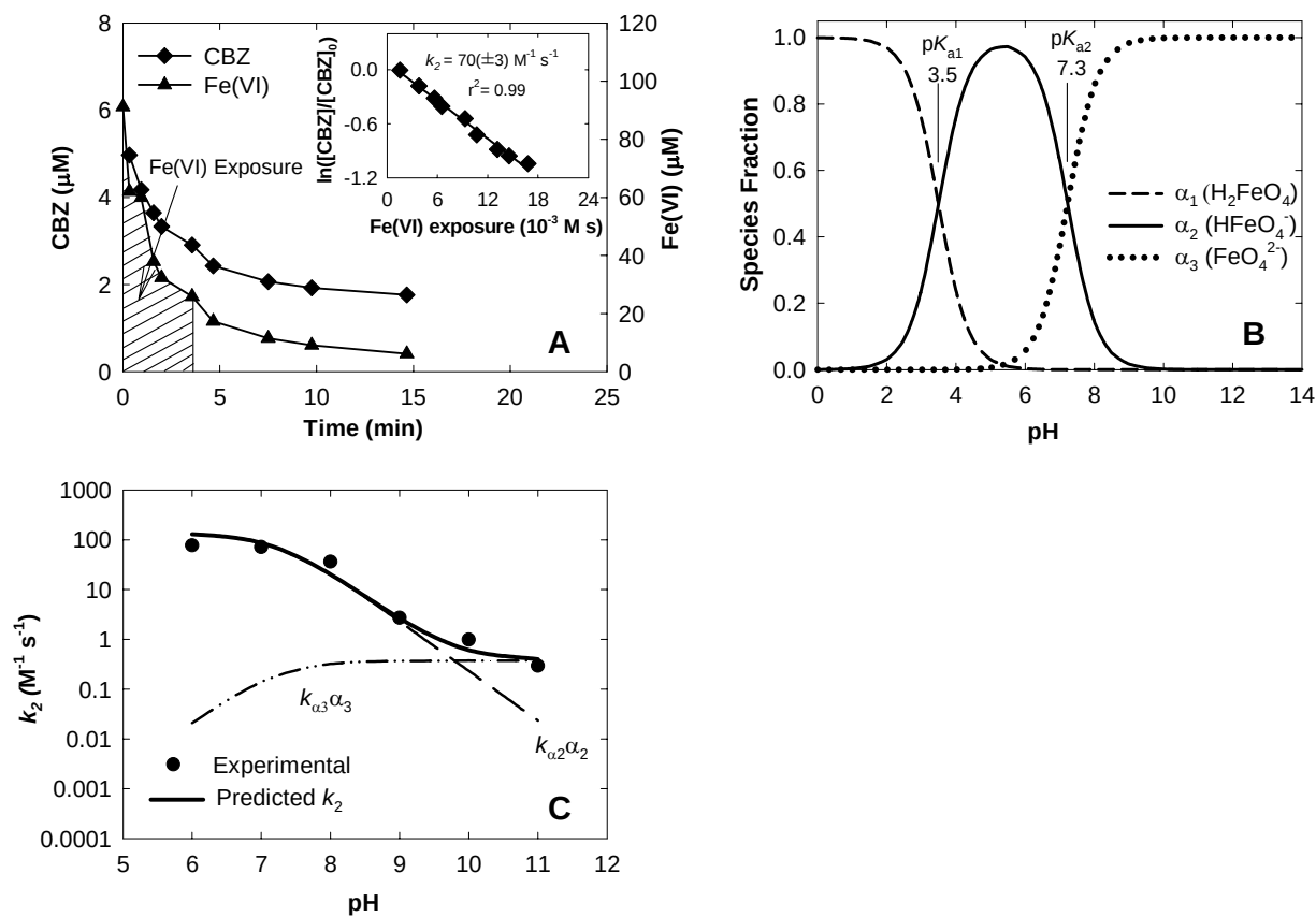
Figure 2.6. Kinetics of CBZ-Fe(VI) reactions. (A) CBZ and Fe(VI) degradation in a batch reaction ( [CBZ]_0 = 5 \text{ } \mu\text{M} , [Fe(VI)]_0 = 100 \text{ } \mu\text{M} , pH 7, 25 mM phosphate buffer, 25 °C). Inset shows fit of batch kinetic data from panel A using Equation (2.6), (B) calculated Fe(VI) speciation versus pH, (C) effect of pH on rate constants for CBZ-Fe(VI) reactions and associated model fit (pH 6–11, [CBZ]_0 = 5 \text{ } \mu\text{M} , [Fe(VI)]_0 = 100 \text{ } \mu\text{M} , 25 mM phosphate buffer (+5 mM borate buffer for pH 9–11 at 25 °C). The solid line in panel C depicts the model fit results, and dashed lines show predicted contributions of reactions with \text{HFeO}_4^- and \text{FeO}_4^{2-} to the overall k_2 values measured at different pH conditions.
