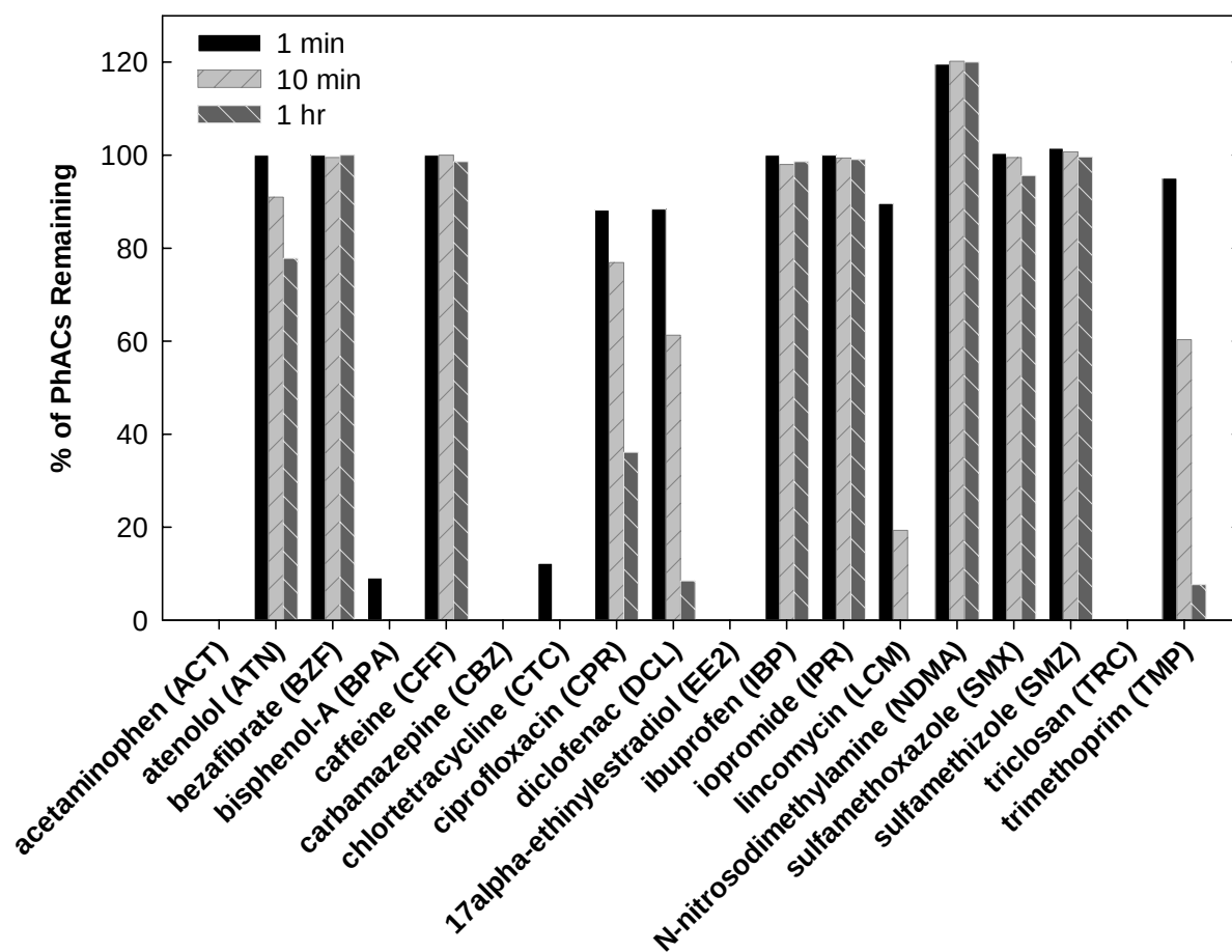
Figure 1.2 Survey results of PhAC reactivity with Mn(VII). Individual bars represent the percent of each PhAC remaining after treatment with Mn(VII) for 1 min, 10 min and 1 h. Reaction conditions: [\text{Mn(VII)}]_0 = 500 \mu\text{M} , [\text{PhAC}]_0 = 10 \mu\text{M} , 25^\circ\text{C} , pH 8.0 (10 mM bicarbonate buffer).
