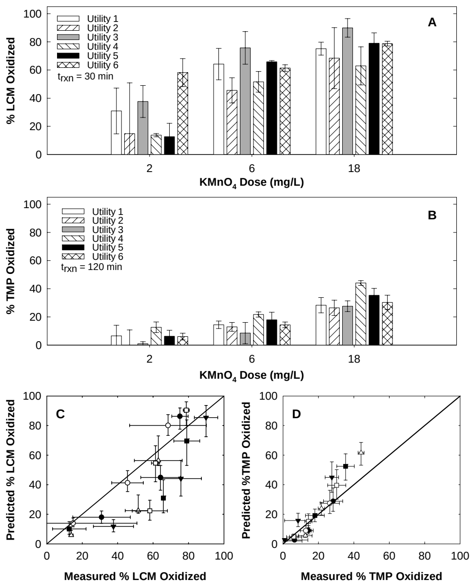
Figure 3.6. Measured oxidation of (A) LCM and (B) TMP during Mn(VII) treatment in six utility source waters at varying applied \text{KMnO}_4 dosages. Comparison of measurements and model predictions with Equation (3.5) for (C) LCM and (D) TMP. Conditions: [\text{ATB}]_0 = 10 \mu\text{g/L} , pH unadjusted (see Table 3.3), room temperature, t_{\text{rxn}} = 30 \text{ min} (LCM) and 120 min (TMP). Uncertainties for measured values are triplicate-averaged 95% confidence levels, and uncertainties for predicted values are obtained by assuming \pm 0.2 \text{ pH} and \pm 1 \text{ }^\circ\text{C} uncertainties. Different symbols in panels C and D refer to experiments conducted in different source waters.
