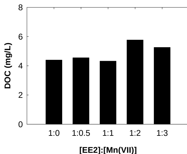
Figure 5.4. Measured dissolved organic carbon (DOC) concentration of EE2 solutions after treatment with different doses of Mn(VII). Reaction conditions: [\text{EE2}]_0 = 18 \text{ }\mu\text{M} , varying [\text{Mn(VII)}] , pH 7, room temperature.
