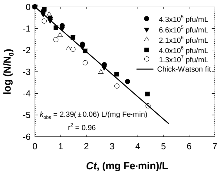
Figure 6.2. Effect of initial MS2 phage concentration on the inactivation kinetics at pH 7 and 25 °C. Experimental conditions are listed in Table 6.1. The line and k_{\text{obs}} shown are from a single regression with the five data sets combined. Uncertainty represents 1 \sigma .
