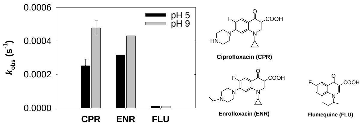
Figure 3.3. Reactivity of ciprofloxacin and structurally related fluoroquinolones with Mn(VII) at pH 5 and pH 9. Conditions: [fluoroquinolone] _0 = 10 \mu M, [Mn(VII)] _0 = 500 \mu M, 25 mM phosphate buffer, 25 ^{\circ} C.
