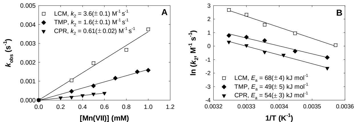
Figure 3.2. Effect of (A) Mn (VII) concentration and (B) temperature on measured rate constants for oxidation of antibiotics. Reaction conditions. [\text{CPR}]_0 = 10 \mu\text{M} , [\text{LCM}]_0 = 20 \mu\text{M} , [\text{TMP}]_0 = 10 \mu\text{M} , 25 mM phosphate buffer, pH 7, 25^\circ\text{C} for (A); [\text{CPR}]_0 = 10 \mu\text{M} , [\text{LCM}]_0 = 20 \mu\text{M} , [\text{TMP}]_0 = 10 \mu\text{M} , [\text{Mn(VII)}]_0 = 500 \mu\text{M} , 25 mM phosphate, pH 7 for (B). Lines represent linear regressions of measured data. Uncertainties represent 1 \sigma .
