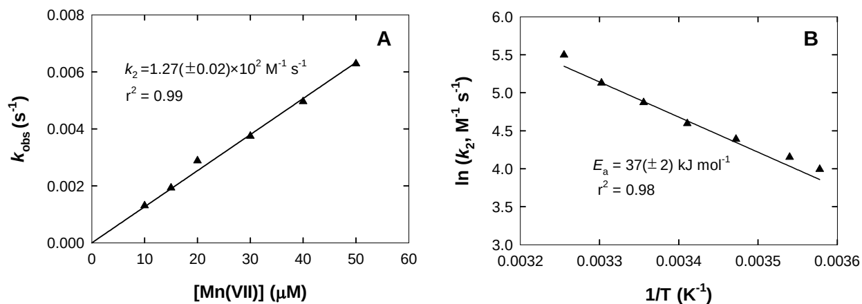
Figure 5.2. Effects of (A) Mn(VII) concentration and (B) temperature on rate constants of EE2 reaction with Mn(VII). Experimental conditions: [EE2]_0 = 1 \text{ } \mu\text{M} , 25 mM NaCl, pH 7, 25 \text{ } ^\circ\text{C} for (A); [EE2]_0 = 1 \text{ } \mu\text{M} , [Mn(VII)]_0 = 10 \text{ } \mu\text{M} , 25 mM NaCl, pH 7 for (B). Lines represent linear regressions of measured data. Uncertainties represent 1 \sigma .
