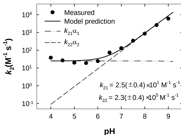
Figure 5.3. Effect of pH on measured and model-predicted rate constants for Mn(VII) reactions with EE2. [\text{EE2}]_0 = 1 \text{ }\mu\text{M} , [\text{Mn(VII)}]_0 = 10 \text{ }\mu\text{M} , 25 mM NaCl, 25 °C. Symbols represent measurements and lines indicate overall model predictions. Uncertainties represent 1 \sigma .
