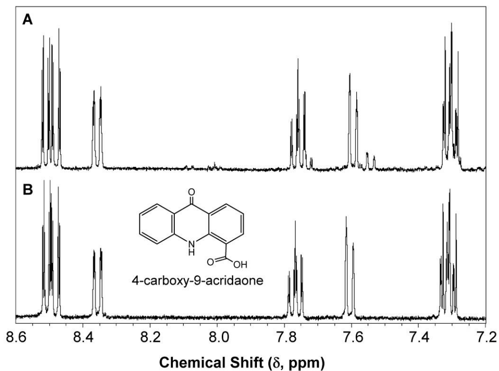
Figure 2.1. Aromatic region of ^1\text{H} -NMR spectra of (A) isolated final product from CBZ-Mn(VII) reaction, and (B) 4-carboxy-9-acridanone reference standard. The spectra agree closely, with the exception of a few additional small peaks in the sample isolated from the reaction mixture, which are presumed to be due to impurities in the solid phase extract.
