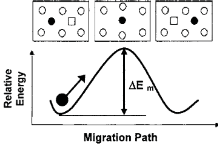
Figure 3.2: Defect energy along the oxygen migration pathway [32]. Migration energy is calculated as the difference between the saddle point and minimum energies.
