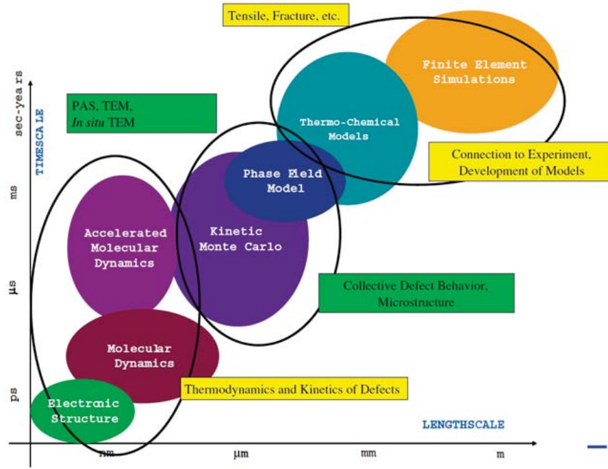
Figure 2.2: Visualization of computational modeling techniques shown over the length and time scales that they apply to [9].
