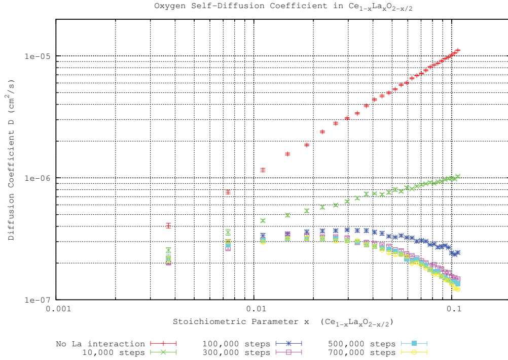
Figure 5.5: KMC simulation steps comparison using migration energies derived from the Gotte [23] potential.
