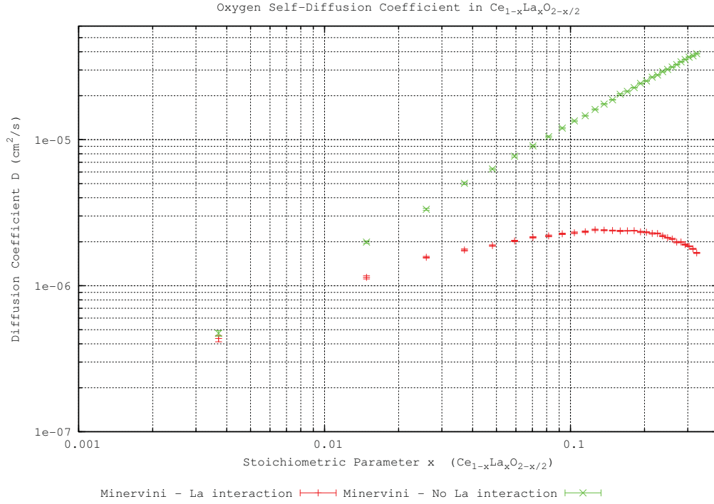
Figure 5.7: KMC simulation results for migration energies derived from the Minervini [7] potential.
