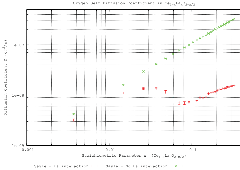
Figure 5.8: KMC simulation results for migration energies derived from the Sayle [24] potential.
