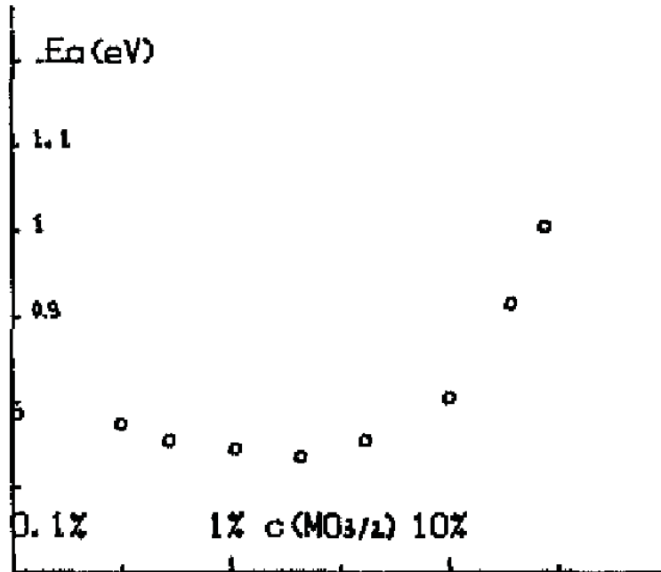
Figure 5.9: Effective activation energy as a function of non-stoichiometry in La-doped ceria [38].
