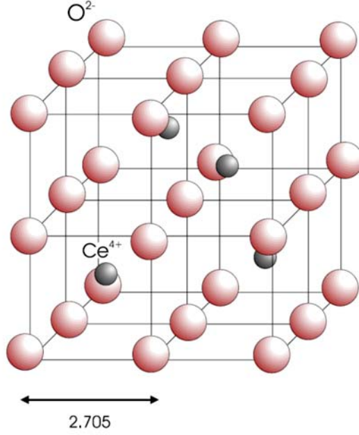
Figure 2.1: Schematic representation of \text{CeO}_2 (fluorite) unit cell.
