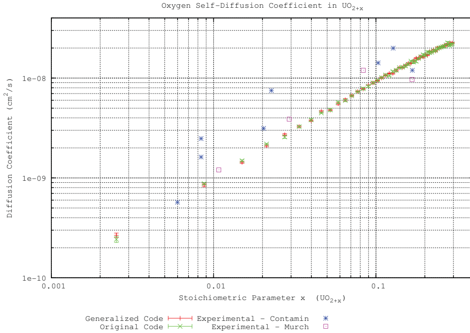
Figure 5.3: Comparison of calculated and experimentally measured oxygen self-diffusivities in hyperstoichiometric UO_2 .
