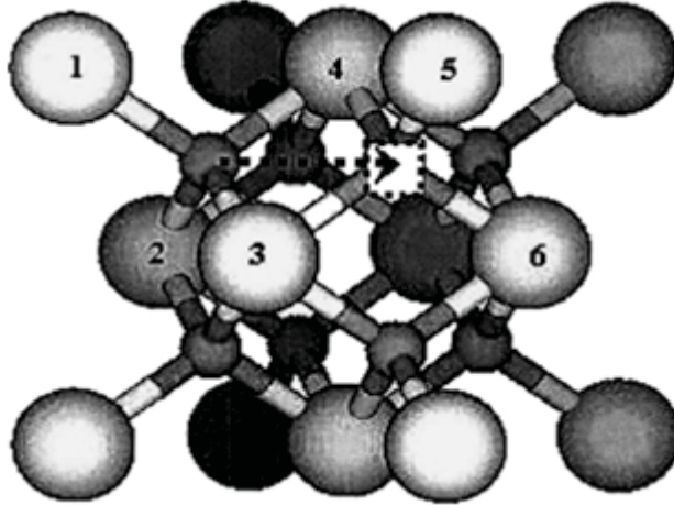
Figure 3.1: Schematic representation of the migrating vacancy and local dopant environment used to model vacancy migration in La-doped \text{CeO}_2 [32]. The arrow shows the migration pathway of the oxygen atom (opposite pathway of the oxygen vacancy), the square shows the initial position of the vacancy before migration, and the six numbered cation sites show the local configuration sites that are considered.
