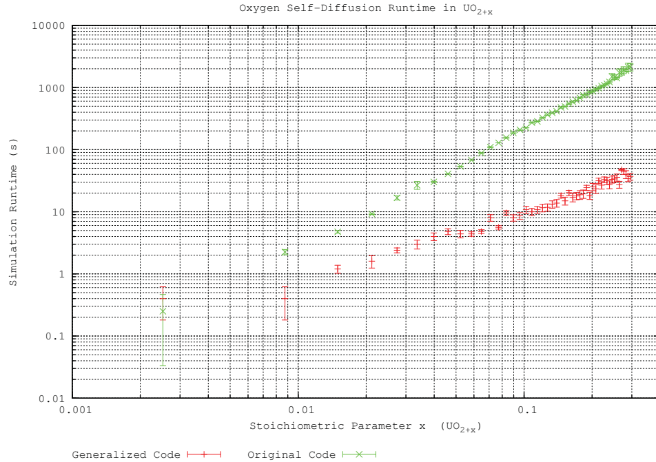
Figure 5.2: Comparison of computational complexity with respect to the particle count (shown here as a function of the stoichiometric parameter) shown on a logarithmic scale for accurate comparison of runtime values.
