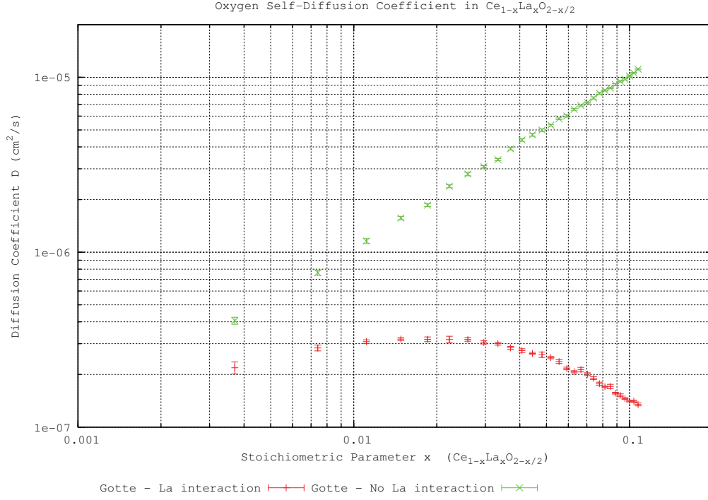
Figure 5.6: KMC simulation results for migration energies derived from the Gotte [23] potential.
