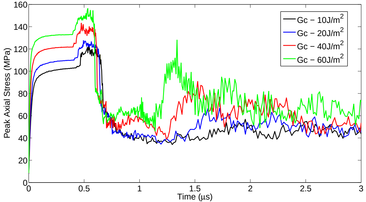
Figure 4.12 – Effect of fracture toughness G_c on the evolution of the peak axial stress in a 5 \mu m -thick PI film with varying interface strength \sigma_c .
