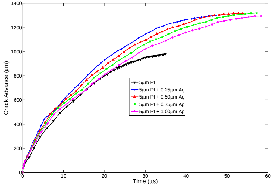
Figure 4.8 – Comparison of the crack advances obtained for a 5 \mu m -thick PI film with Ag inertial layers of varying thickness ranging from zero to 1 \mu m . The inertial layer is seen to help improve the crack advance by about 310 \mu m .
