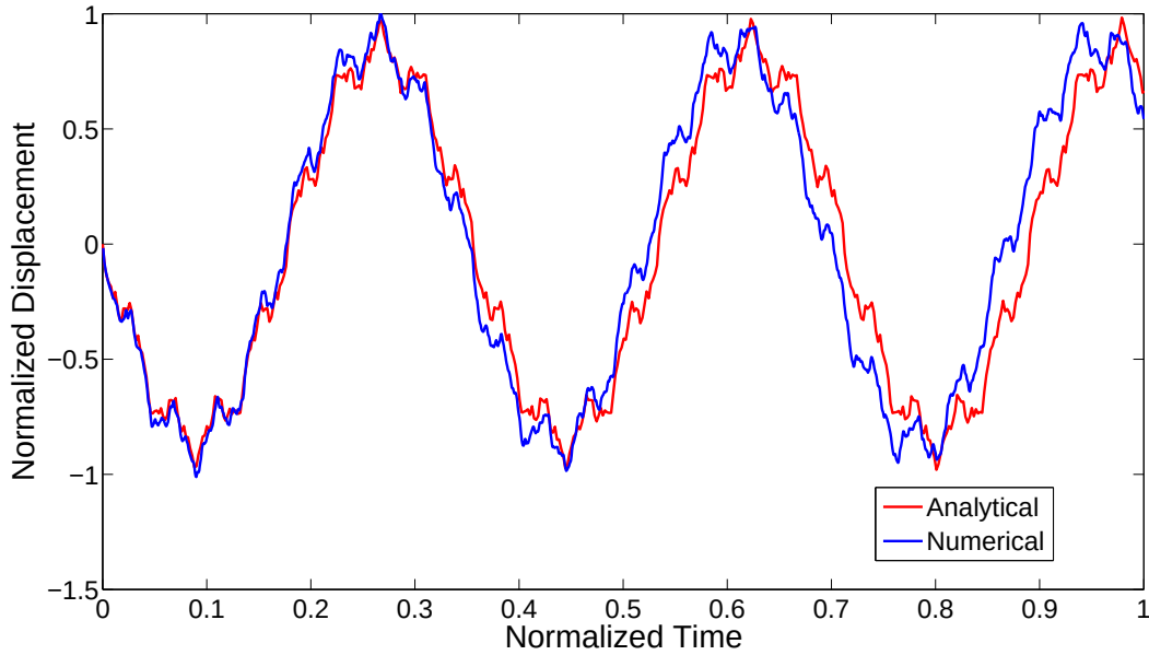
Figure 3.4 – Dynamic verification problem: normalized dynamic deflection of an axially pre-stressed beam (with an axial resultant load of 10,000 N ) loaded with an impulse transverse load of 1000 N . Good agreement is obtained between analytical and numerical results.
