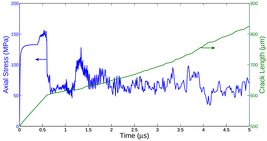
Figure 4.9 – Comparison of the crack advance and axial stress evolution for a 5 \mu m -thick PI film with an Au inertial layer of 100 nm . The axial stress peaks during initial lift-off of the pre-crack region, which is characterized by higher crack tip velocities as well.
