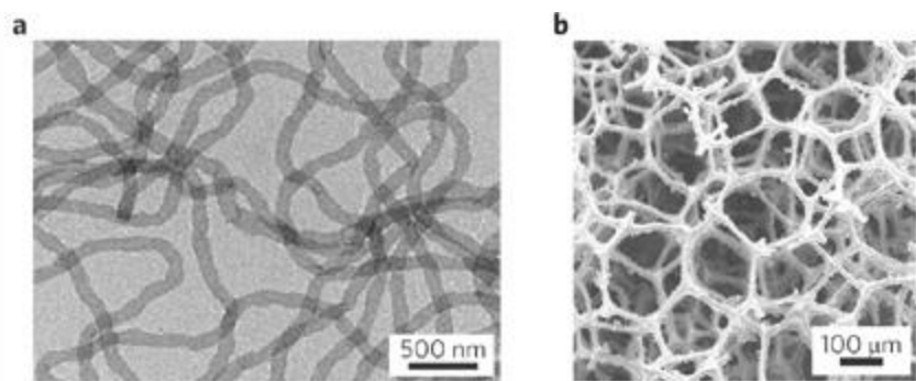
Figure 2.4. Use of self-organized media. TEM image showing SiO 2 -polymer nanotubes formed by myelination of poly(ethylene oxide)- b -poly(1,2-butylene oxide)-tetraethoxysilane gel particles in water ( a ), and scanning electron microscopy (SEM) image showing a polyhedral framework of zeolite and SiO 2 nanoparticles produced by microphase separation and spatial patterning within the interstitial voids of a dextran-derived foam of CO 2 gas bubbles ( b ). Reprinted from Mann (2009). Reprinted from Nature Materials; S. Mann; Self-assembly and transformation of hybrid nano-objects and nanostructures under equilibrium and non-equilibrium conditions; pages 781-792; copyright 2009; with permission from Nature Publishing Group, U.S.A.
