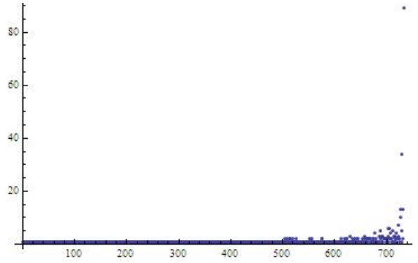
Figure 4.10: Length of gaps for the 14th row
