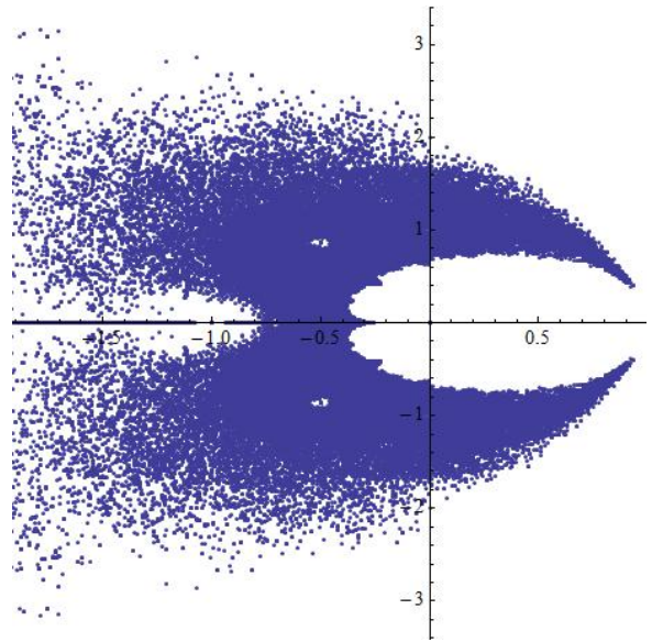
Figure 11.2: Zeros of \hat{w}(n, x) up to n = 2^{15}
