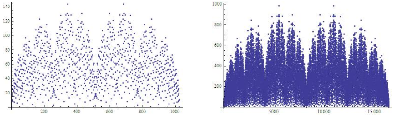
Figure 4.3: Values for the 10th and 14th rows of s(n)
