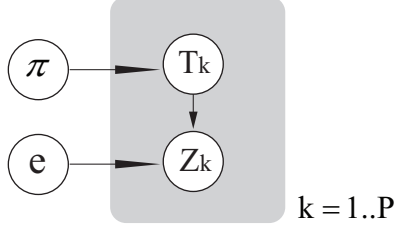
Figure 10.2: The epitome graphical model.
