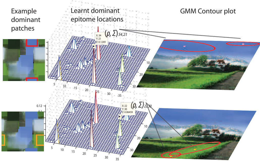
Figure 6.1: A 36 \times 36 spatialized epitome (in the first column) is learned from the image in the third column. The distribution in the middle column shows the positions of the significant patches. Note that most locations are of zero value due to regularization. The leftmost image in each row highlights a significant patch in the spatialized epitome. Its associated Gaussian mixture which represents the spatial arrangement of the significant patch in the input image is shown as ellipse contours in the third column.
