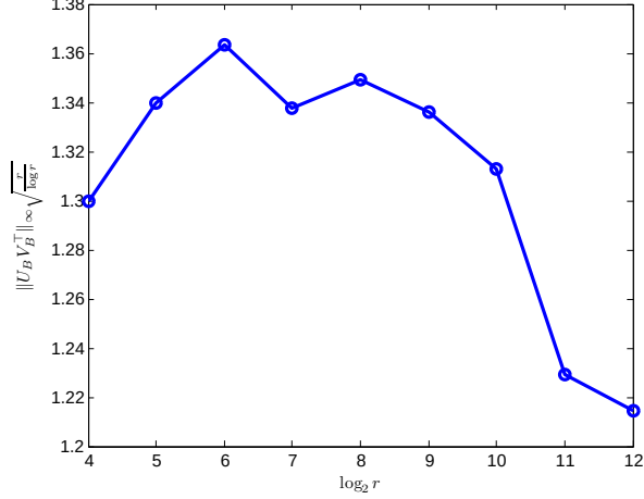
Figure 3.2: Simulation result supporting Conjecture 3.1. The conjecture is equivalent to \|U_B V_B^\top\|_\infty = \Theta(\sqrt{\frac{\log r}{r}}) .
