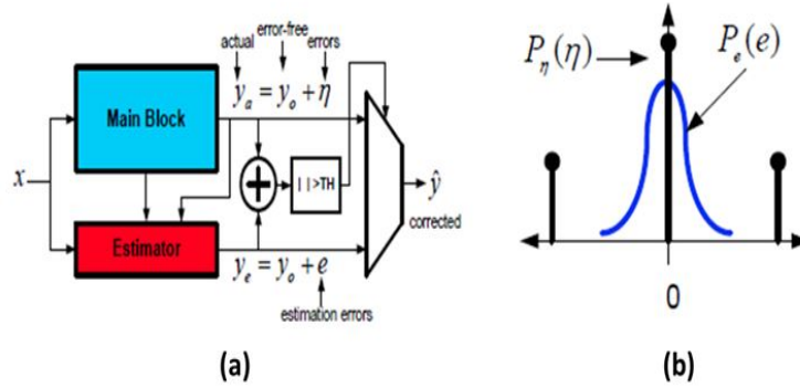
Figure 3.2: Algorithmic noise-tolerance: (a) block diagram for ANT-based design, and (b) desired error distributions for ANT [29].
