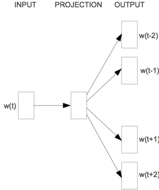
Figure 3.1: Skip-gram Model
