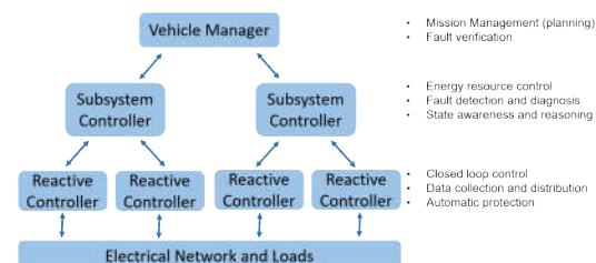
Fig 2. Generalized Hierarchical Autonomous Control Architecture
