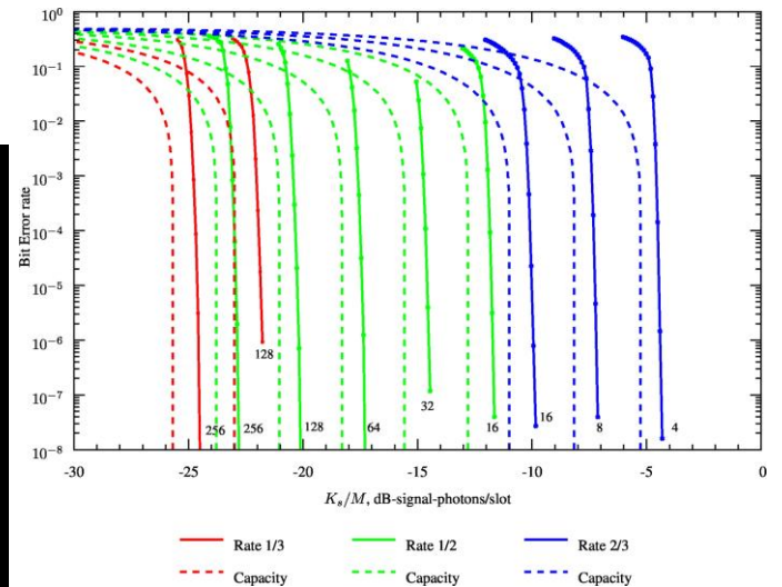
Figure 4: SCPPM performance, for Kb=0.01
