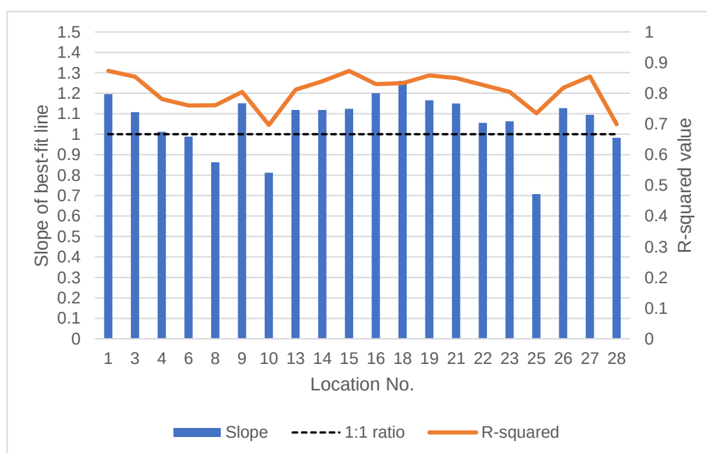
Figure 5. Slope and R^2 for the linear best-fit line between hourly T_{air} measurements and LST from Landsat imagery. The “best-fit” 1:1 ratio level is shown as a dashed horizontal line.
