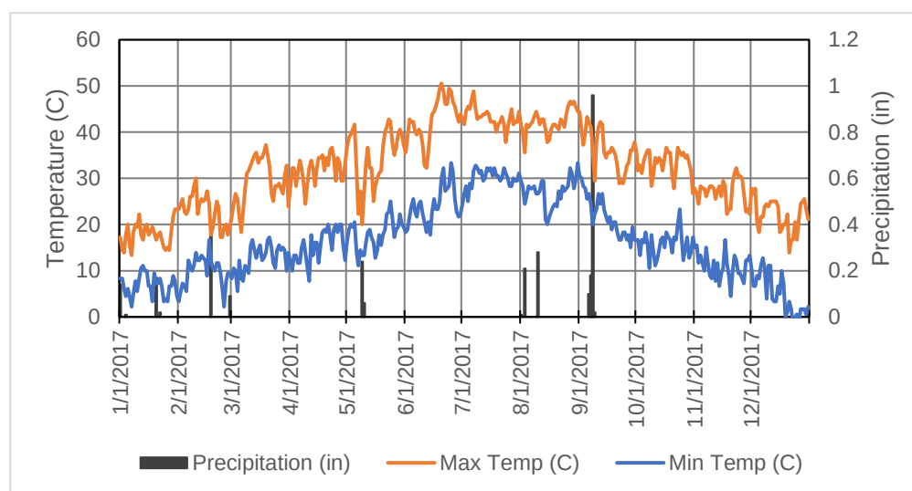
Figure 2. Climatology from Ford Dry Lake SCAN station in 2017
