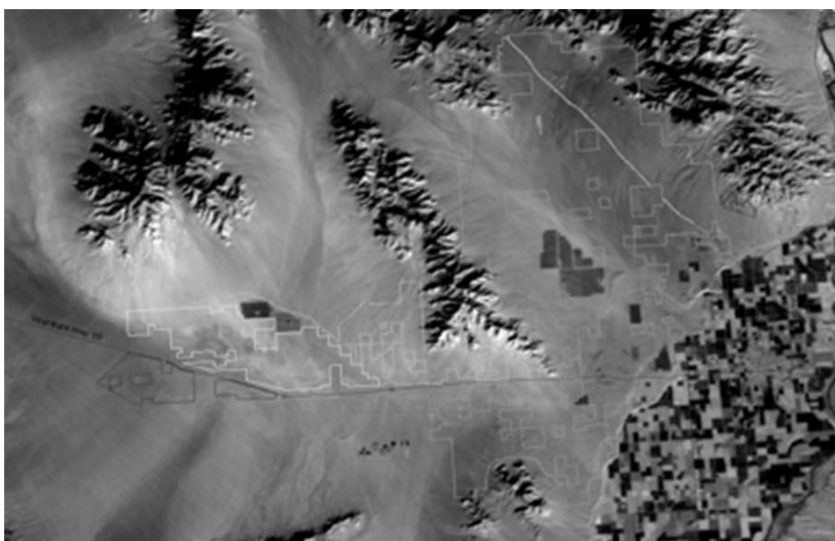
Figure 7. June 2016 Landsat LST grayscale image, centered on the Valen and McCoy Wilderness Area in eastern Riverside County and the solar energy development zones shown in white outlines. LST ranges from 40°C in black shades to 50°C in light gray shades.
