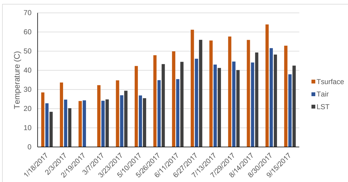
Figure 6. Comparison of T_{\text{surface}} , T_{\text{air}} , and LST at the hour of Landsat flyover for a selected measurement location.
