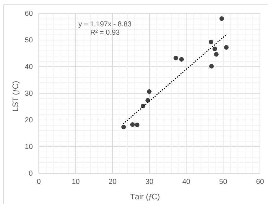
Figure 4. Scatter plot between T_{air} , and 2017 Landsat LST image data for measurement location 1 in Ford Dry Lake.
