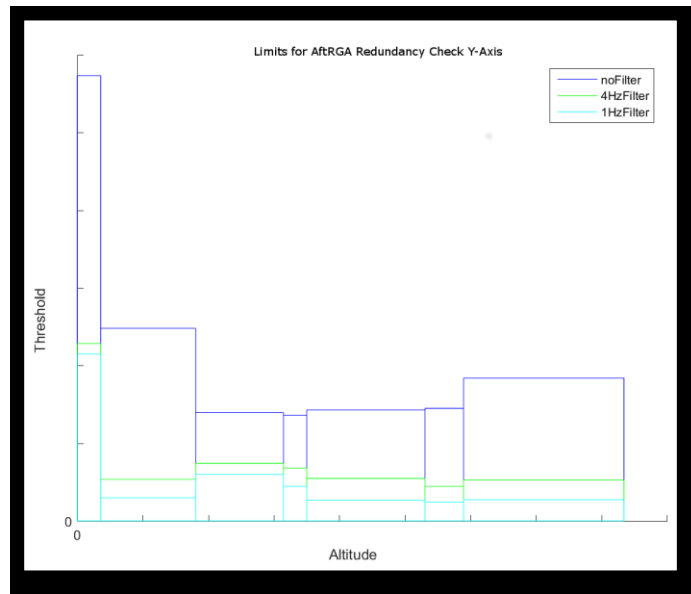
Figure 4 Effects of using a low-pass filter on the angular rate measurements in the Redundancy Check.
