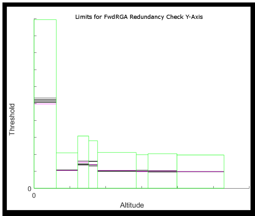
Figure 3 The zero-margin thresholds for each altitude phase along with the scaled thresholds used across all configurations.
