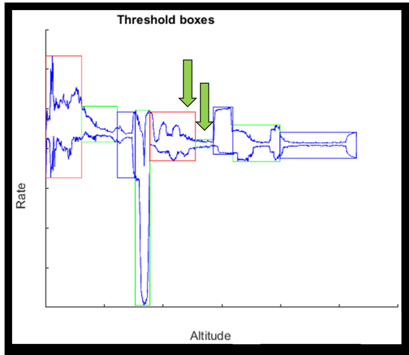
Figure 2 The minimum and maximum pitch rate versus altitude data along with the altitude-based SDQ flight phases. The two indicated phases were merged using the min/max rates across the union of the two sub-intervals.
