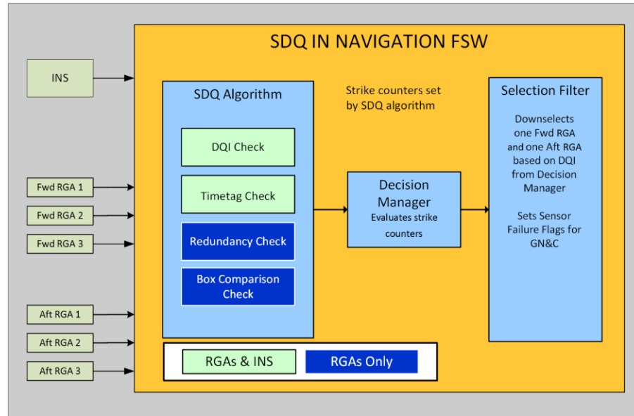
Figure 1- Data flow through navigation SDQ.
