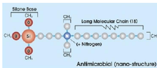
Fig. 2. Quat-silane working mechanism [33].
