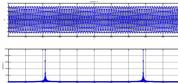
Figure 2 : Atomic Interaction
