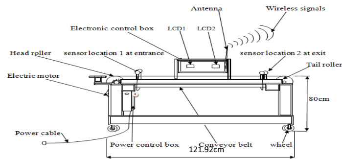
Figure 1: Machine structure
