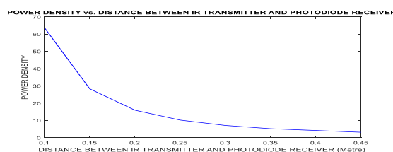
Figure 6: A graph of Effect of distance between sensors on power density
