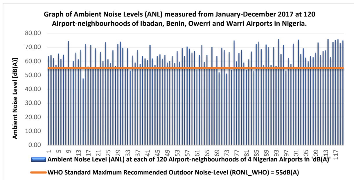
Figure 6: Graph of Ambient Noise Levels (ANL) measured from January-December 2017 at 120 Airport-neighbourhoods of Ibadan, Benin, Owerri and Warri Airports in Nigeria.
