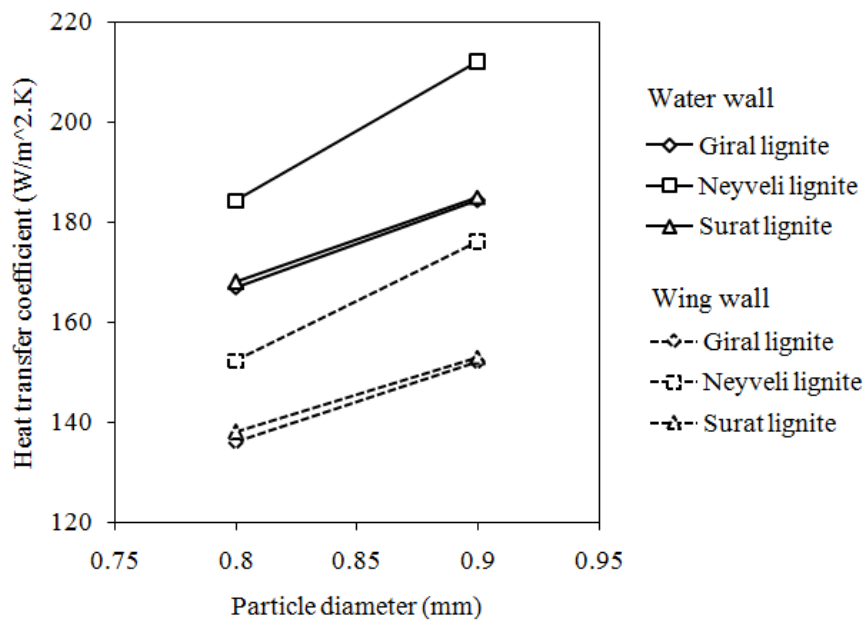
Figure 7. Projected water wall heat transfer coefficient at constant bed temperature of 850°C at different particle diameter
