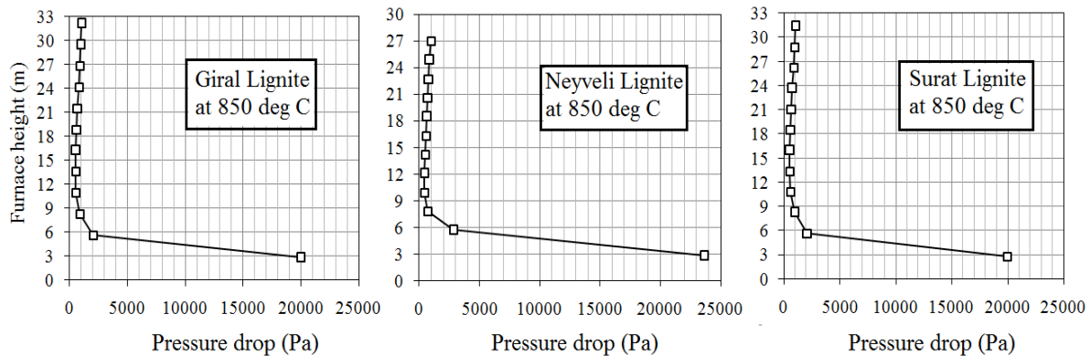
Figure 4. Pressure drop profile along the CFB riser at 0.9mm of mean particle diameter
