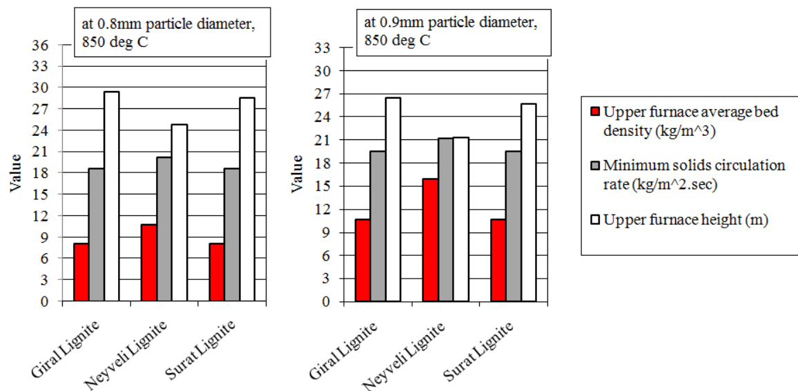
Figure 2. Average bed density, solids circulation rate and upper furnace height at two different particle diameters for three lignite samples
