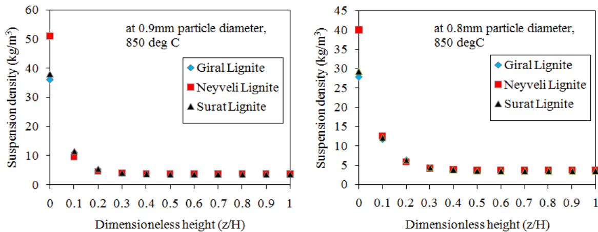
Figure 5. Suspension density profile from the top of the lower furnace to top of the upper furnace
