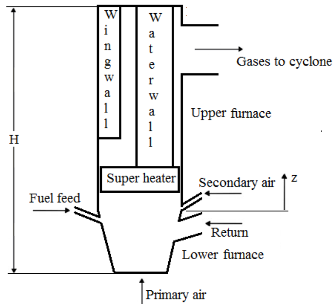
Figure 1. CFB Riser configuration with boiler elements
