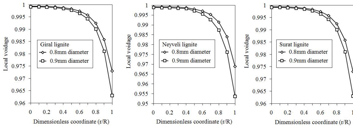
Figure 6. Local voidage profile for three Indian lignite at mean bed voidage of upper furnace
