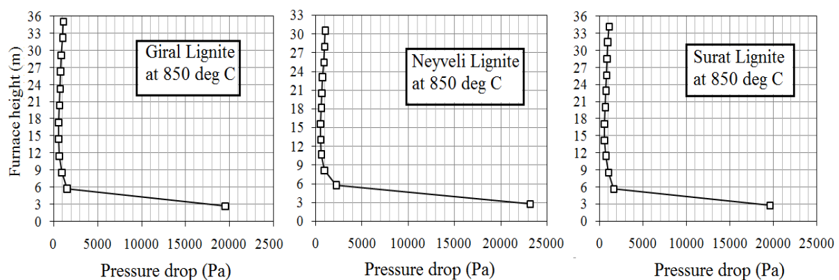
Figure 3. Pressure drop profile along the CFB riser at 0.8mm of mean particle diameter
