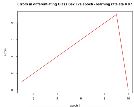
Figure 9. Training Process in Determining Abalone Sex I
