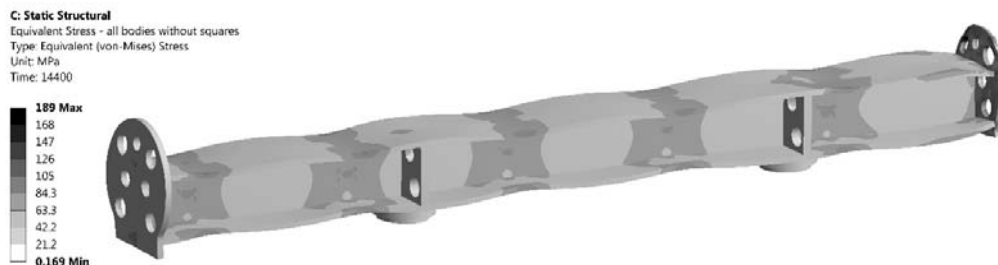
Figure 9. Maximum thermal stress in the support structure (after 4 hours of cooldown).
