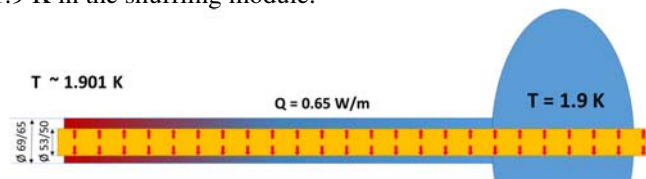
Figure 3. Overview of the calculated maximum temperature of the beam line in operation.
