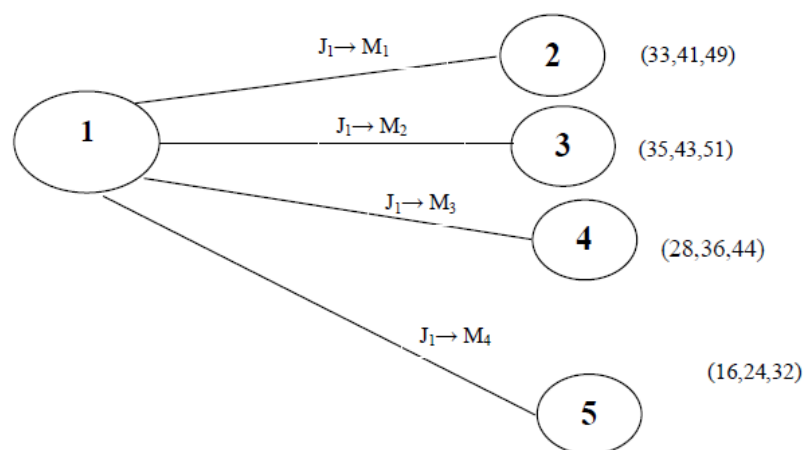
Figure 1. First branch of the solution tree
