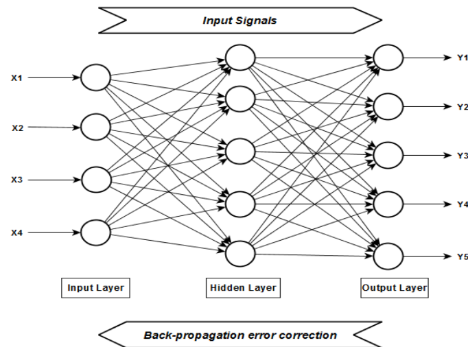
Figure 1. Back propagation model
