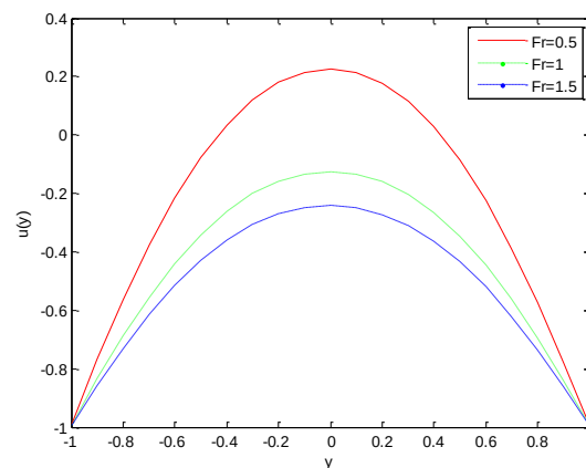
Figure 13. Plot of velocity field u(y) for various values of Fr with a = 0.6 , b = 0.7 , d = 1.5 , R = 2 , \eta = 0.1 , \sigma = 1 , M = 4 , m = 0.03 , x = -0.5 , \phi = \pi/4 , \theta = \pi/3 and dp/dx = 1 .
