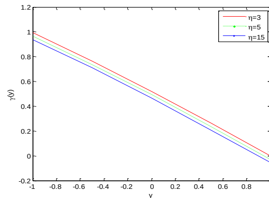
Figure 16. Plot of temperature profile \gamma(y) for various values of \eta with a = 0.6 , b = 0.7 , d = 1.5 , R = 0.5 , M = 4 , Fr = 1.2 , m = 0.03 , x = -0.5 , Du = 0.1 , Sc = 0.5 , Br = Pr = 2 , Sr = 0.6 , \sigma = 1 , \phi = \pi/4 , \theta = \pi/3 and dp/dx = 1 .
