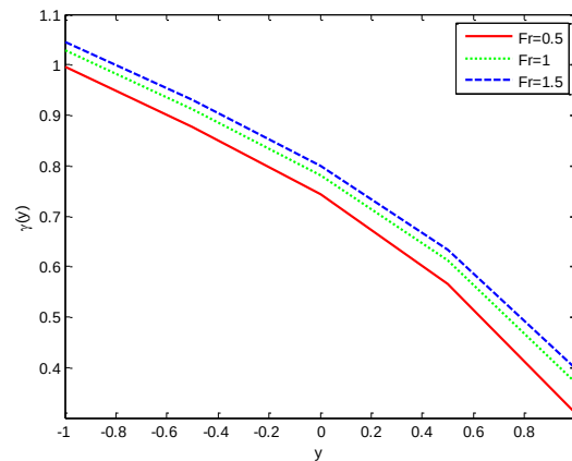
Figure 19. Plot of temperature profile \gamma(y) for various values of Fr with a=0.6 , b=0.7 , d=1.5 , R=0.5 , \eta=0.1 , m=0.03 , \theta=\pi/3 , x=-0.5 , Du=0.1 , Sc=0.5 , Br=Pr=2 , Sr=0.6 , \sigma=1 , \phi=\pi/4 , M=4 and dp/dx=1 .
