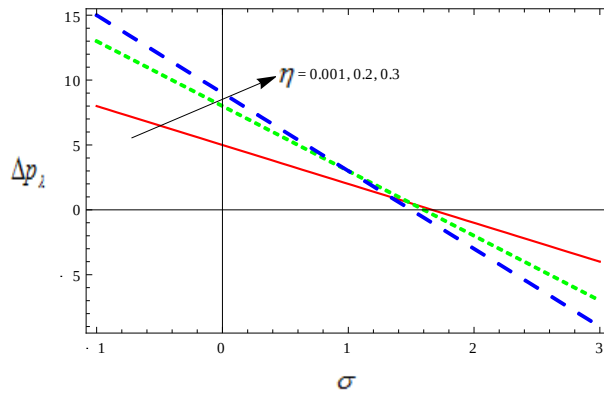
Figure 7. Plot of pressure rise \Delta p_\lambda for various values of \eta with a = 0.7 , b = 1.2 , d = 2 , R = 0.5 , Fr = 1.2 , \phi = \pi/4 , m = 0.03 , M = 4 and \theta = \pi/3 .
