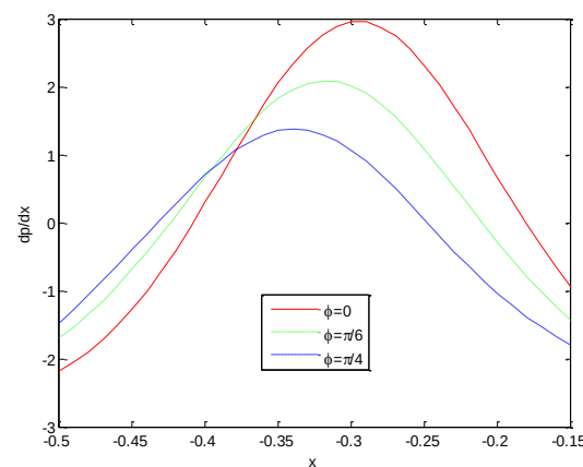
Figure 6. Plot of pressure gradient dp/dx for various values of \phi with a = 0.6 , b = 0.7 , d = 1.5 , R = 0.5 , Fr = 1.2 , \eta = 0.1 , M = 4 , \theta = \pi/3 and m = 0.03 .
