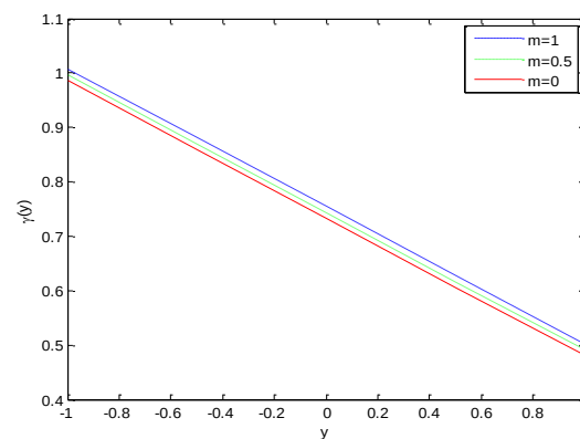
Figure 18. Plot of temperature profile \gamma(y) for various values of m with a = 0.6 , b = 0.7 , d = 1.5 , R = 0.5 , \eta = 0.1 , Fr = 1.2 , \theta = \pi/3 , x = -0.5 , Du = 0.1 , Sc = 0.5 , Br = Pr = 2 , Sr = 0.6 , \sigma = 1 , \phi = \pi/4 , M = 4 and dp/dx = 1 .
