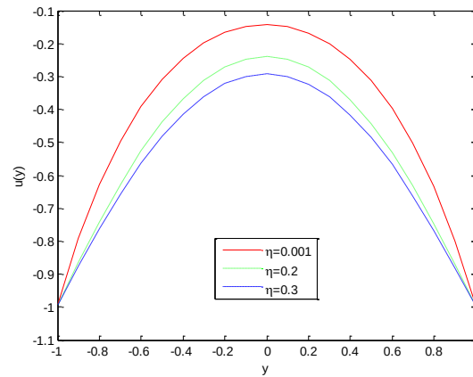
Figure 12. Plot of velocity field u(y) for various values of \eta with a = 0.6 , b = 0.7 , d = 1.5 , R = 2 , Fr = 1.2 , \sigma = 1 , M = 4 , m = 0.03 , x = -0.5 , \phi = \pi/4 , \theta = \pi/3 and dp/dx = 1 .
