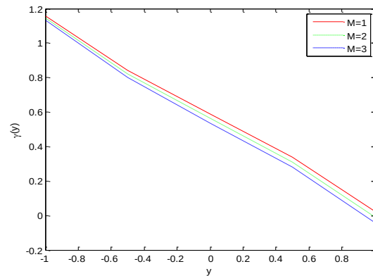
Figure 17. Plot of temperature profile \gamma(y) for various values of M with a = 0.6 , b = 0.7 , d = 1.5 , R = 0.5 , \eta = 0.1 , Fr = 1.2 , m = 0.03 , x = -0.5 , Du = 0.1 , Sc = 0.5 , Br = Pr = 2 , Sr = 0.6 , \sigma = 1 , \phi = \pi/4 , \theta = \pi/3 and dp/dx = 1 .
