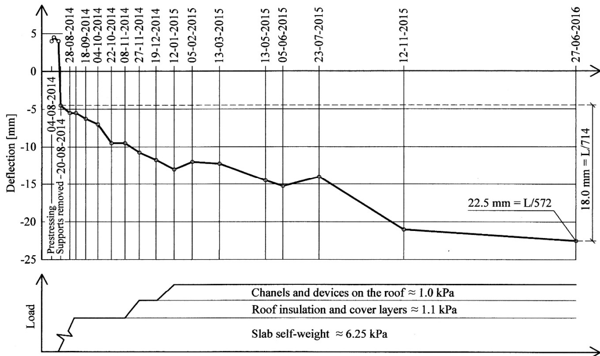
Figure 7. Deflection of roof panel Sl-2.
