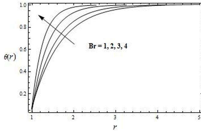
Fig. 12 The Temperature profile for \theta against Br with m = 1, \beta = 0.2, M = 0.5, K = 0.5
