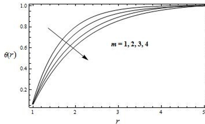
Fig. 13 The Temperature profile for \theta against m with \beta = 0.2, M = 0.5, K = 0.5, Br = 1
