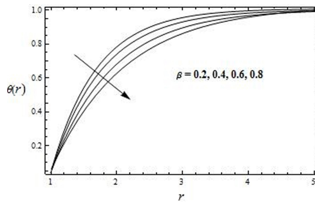
Fig. 11 The Temperature profile for \theta against \beta with m = 1, M = 0.5, K = 0.5, Br = 1
