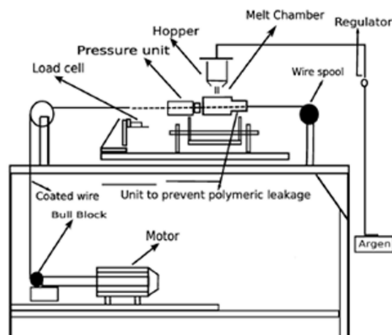
Fig. 1: Emblematic wire coating line
