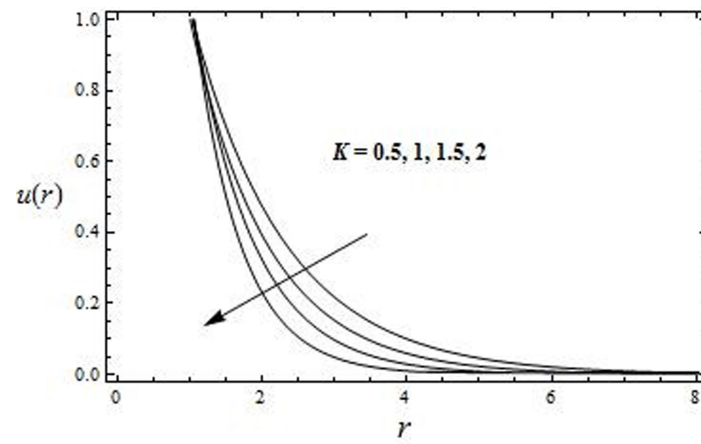
Fig. 6 The velocity profile for u against M with m = 1, \beta = 0.2, M = 0.5
