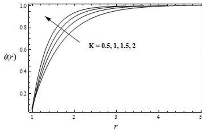
Fig. 10 The Temperature profile for \theta against K with m = 1, \beta = 0.2, M = 0.5, Br = 1
