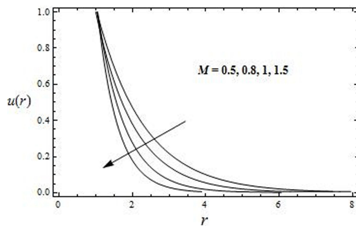
Fig. 5 The velocity profile for u against M with m = 1, \beta = 0.2, K = 0.5
