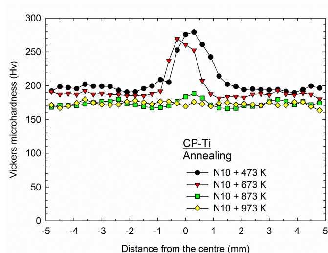
Fig. 4. Distribution of Vickers microhardness, Hv, along the diameter of disc during post-HPT short-term annealing at different temperatures.
