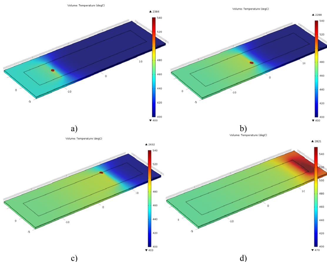
Figure 6. Temperature distribution when scanning a layer at various points of time: 10 s (a); 25 s (b); 40 s (c); 54 s (d).
