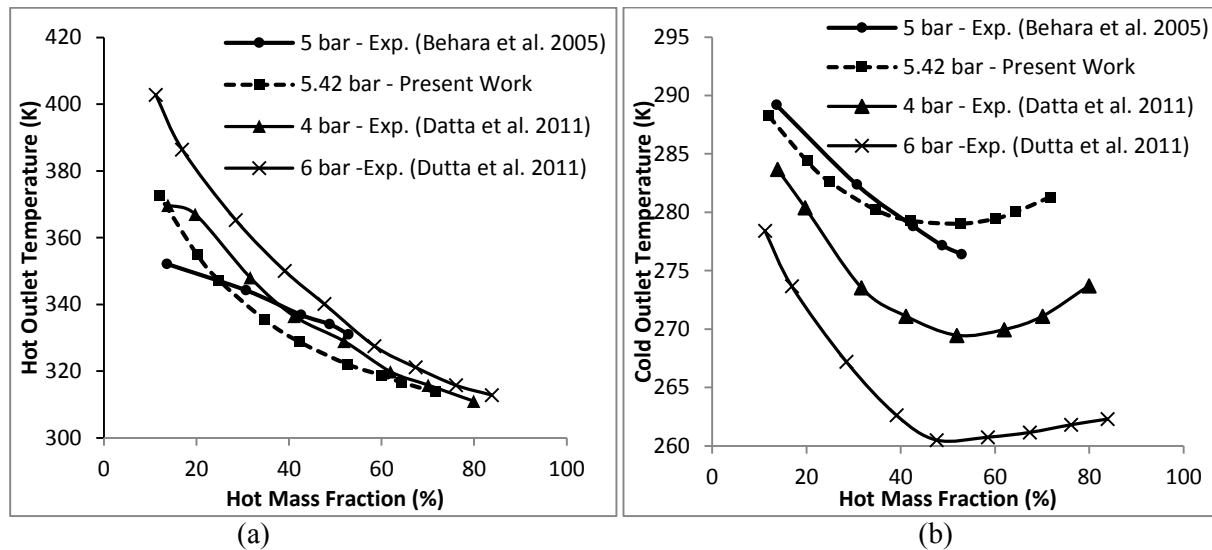
Figure 4. Comparison of experimental and CFD results.
