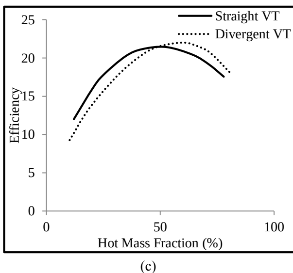
Figure 8. Comparison of (a) COP as refrigerator, (b) COP as Heat Pump and (c) efficiency of straight VT and flared VT.
