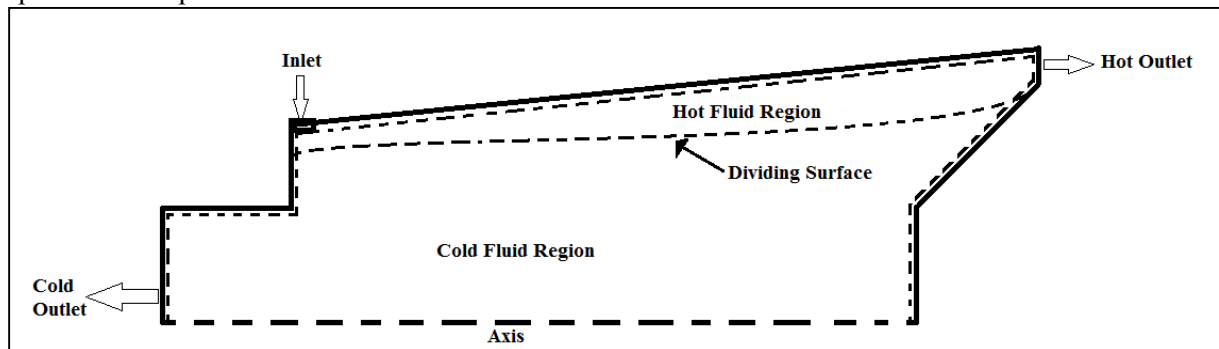
Figure 1. Counter flow flared vortex tube with control volume boundary.
