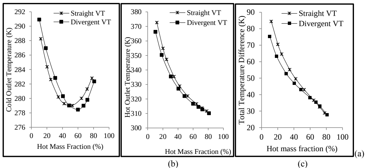
Figure 5. Comparison of (a) cold outlet temperature (b) hot outlet temperature and (c) total temperature difference respectively, with hot mass fraction for both straight and flared tubes.
