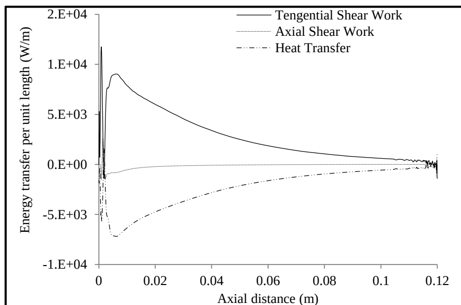
Figure 6. Energy transfer along the axial length at a radial location of 0.005 m.
