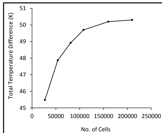
Figure 3. Grid independence study on Total temperature difference.
