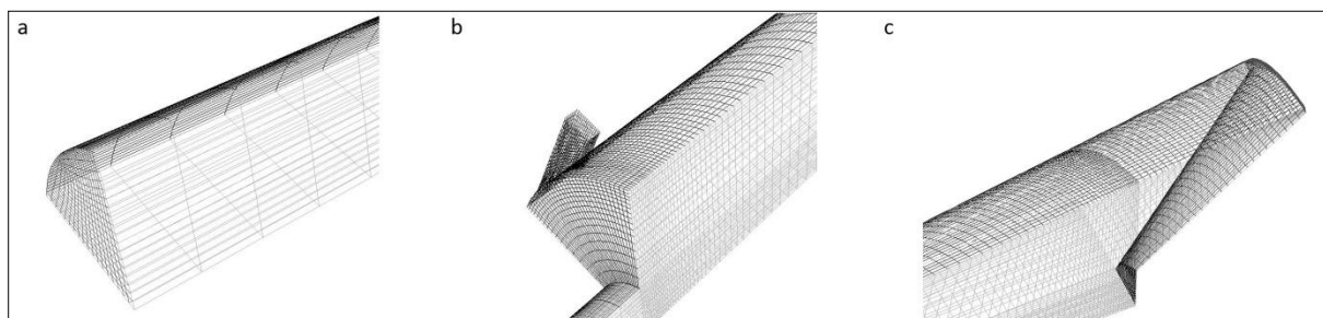
Figure 2. Mesh at (a) cold outlet, (b) inlet and (c) hot outlet of VT
