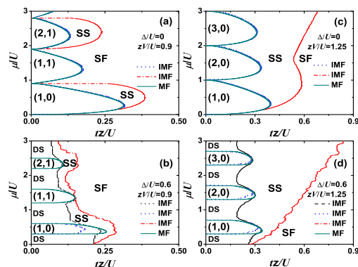
Figure 1. (Color online) The ground-state phase diagrams as a function of the chemical potential \mu/U and hopping tz/U .
